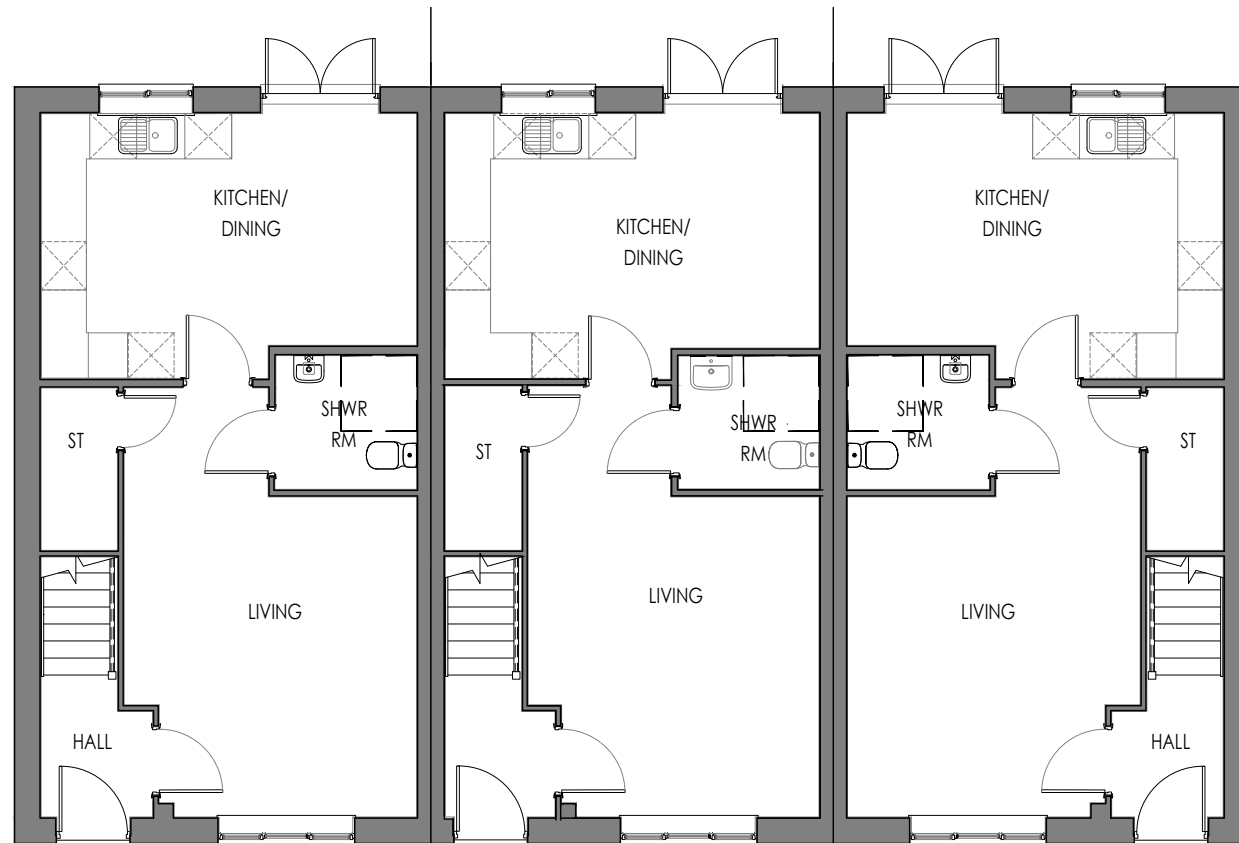
GROUND FLOOR (AS)
