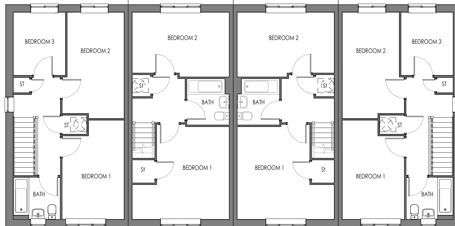
FIRST FLOOR (AS)
