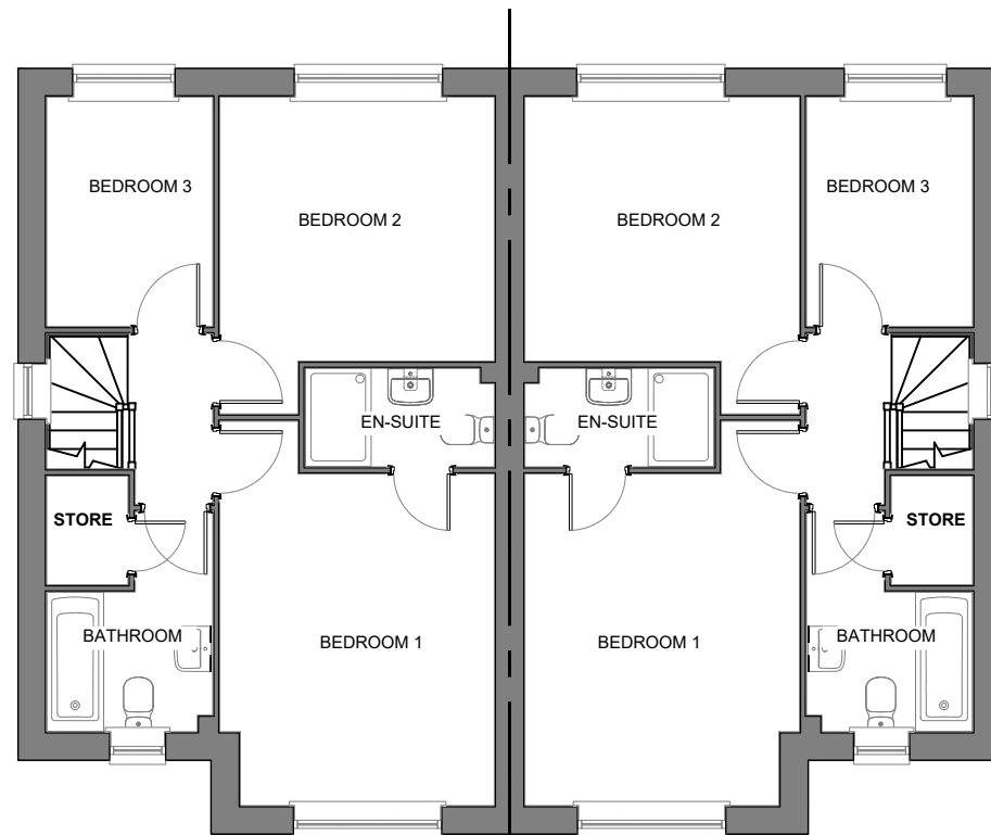
FIRST FLOOR (AS)
