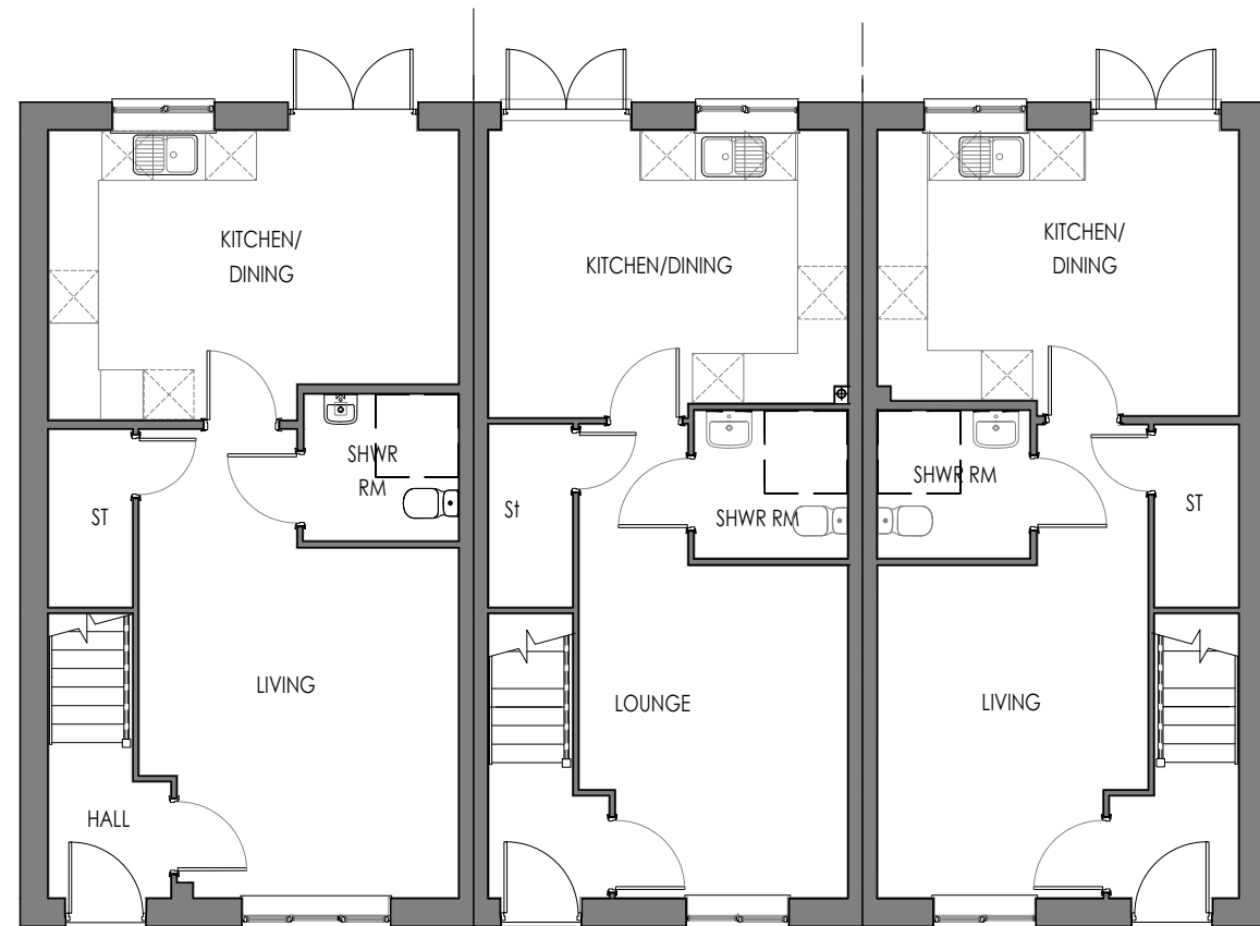
GROUND FLOOR (AS)
