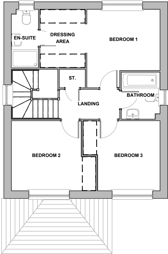
FIRST FLOOR (AS)
