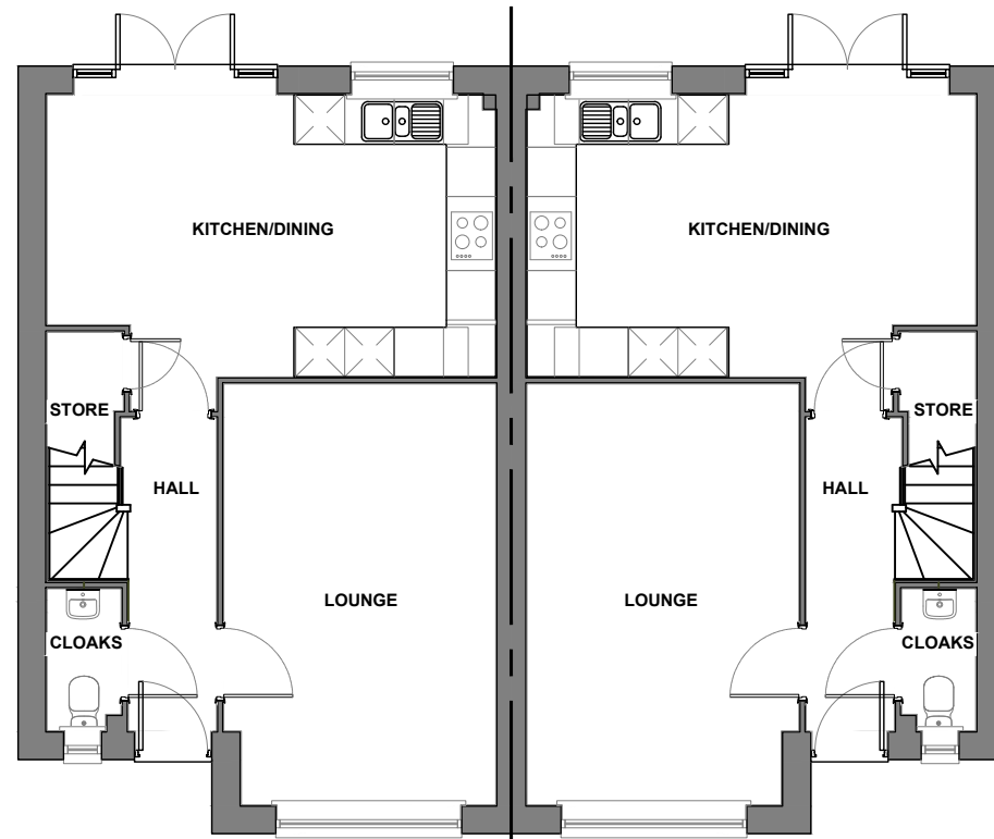
GROUND FLOOR (AS)
