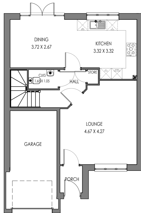
GROUND FLOOR BRO.TF.2 (AS)
