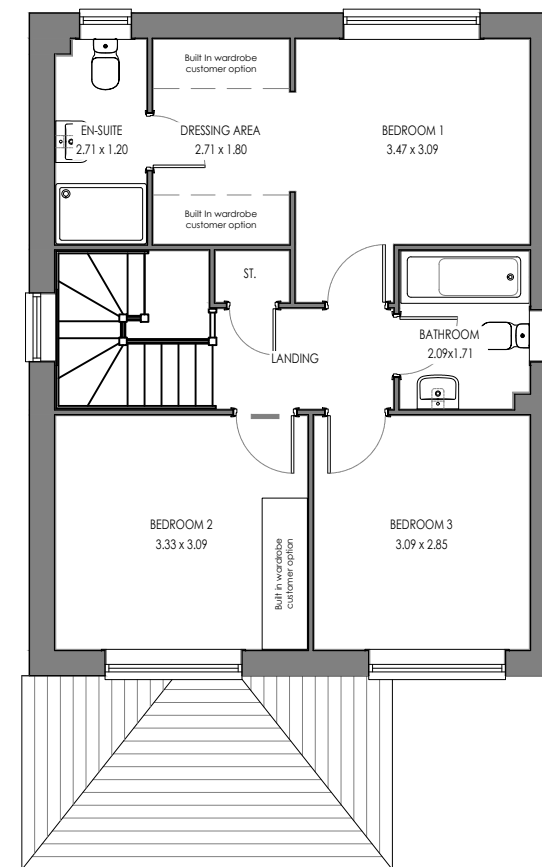
FIRST FLOOR KIN.TF.1 (AS)
