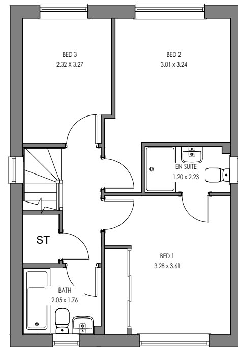
HAR.TF.2 (AS) FIRST FLOOR
