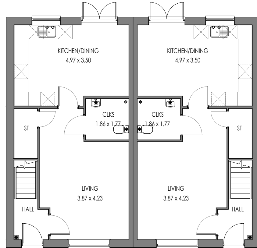
GROUND FLOOR PLAN 5P3B END (AS)
