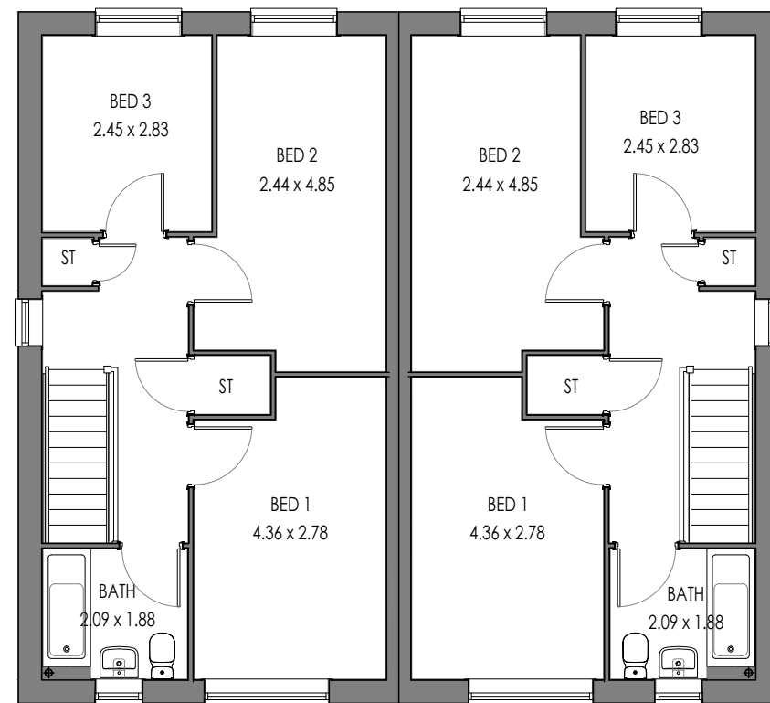
FIRST FLOOR PLAN 5P3B END (AS)
