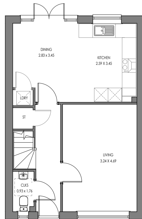
HAR.TF.2 (AS) GROUND FLOOR
