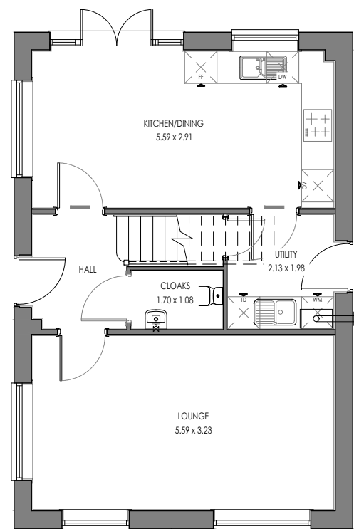
GROUND FLOOR HEN.TF.2 (AS)
