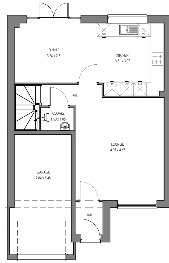
GROUND FLOOR EVE.TF.2 (AS)
