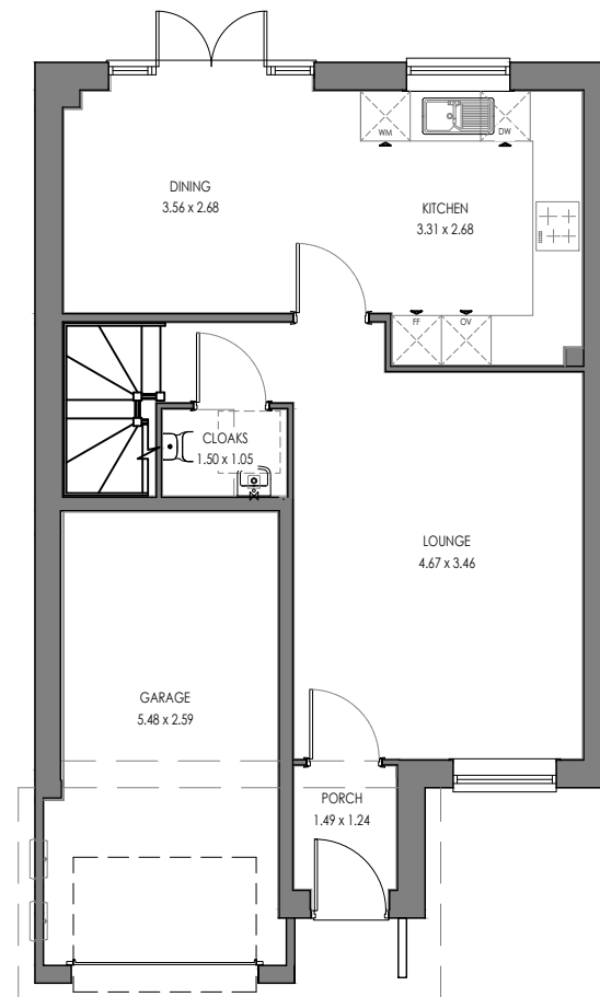
GROUND FLOOR KIN.TF.1 (AS)
