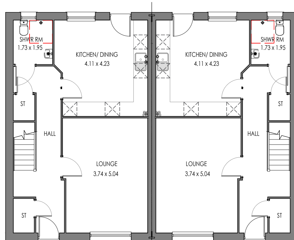
GROUND FLOOR PLAN 6P4B END (AS)
