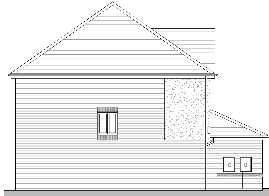
SIDE ELEVATION KIN.TF.1 (AS)
