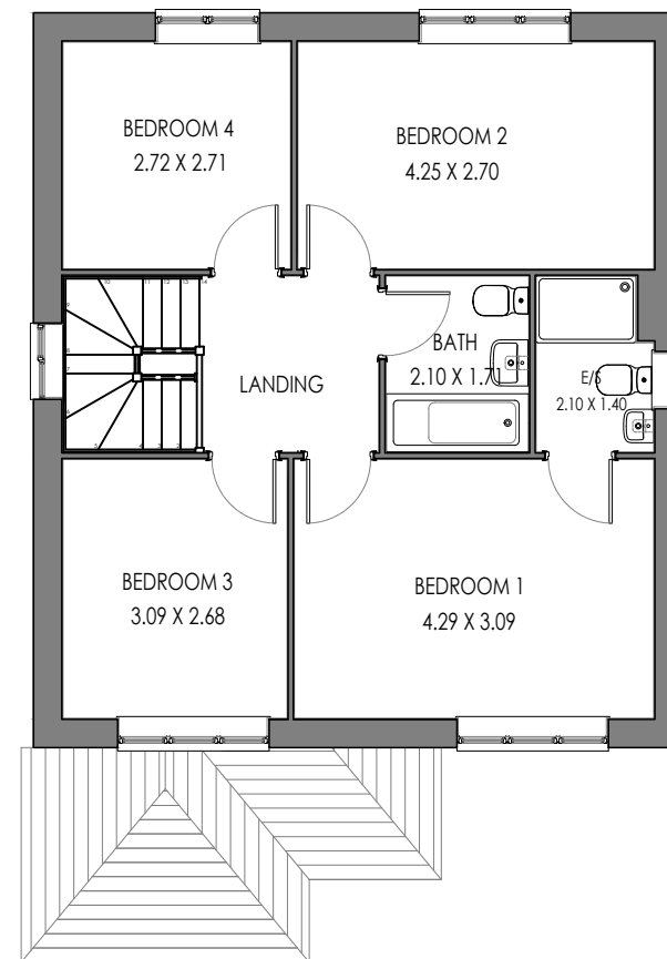
FIRST FLOOR BRO.TF.2 (AS)
