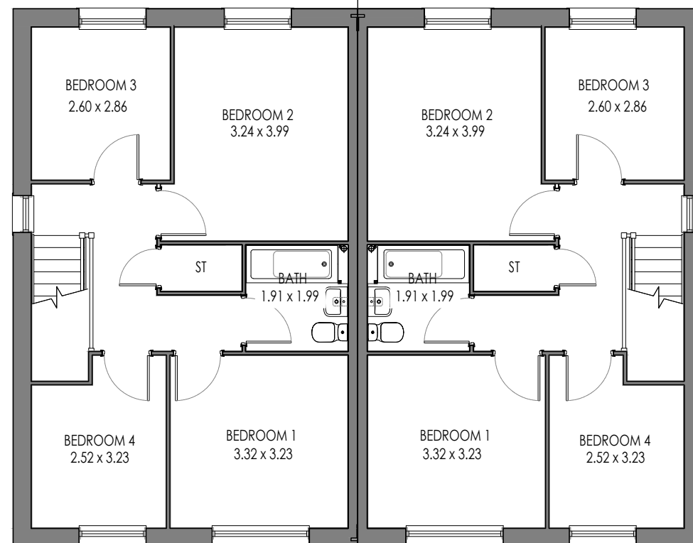
FIRST FLOOR PLAN 6P4B END (AS)
