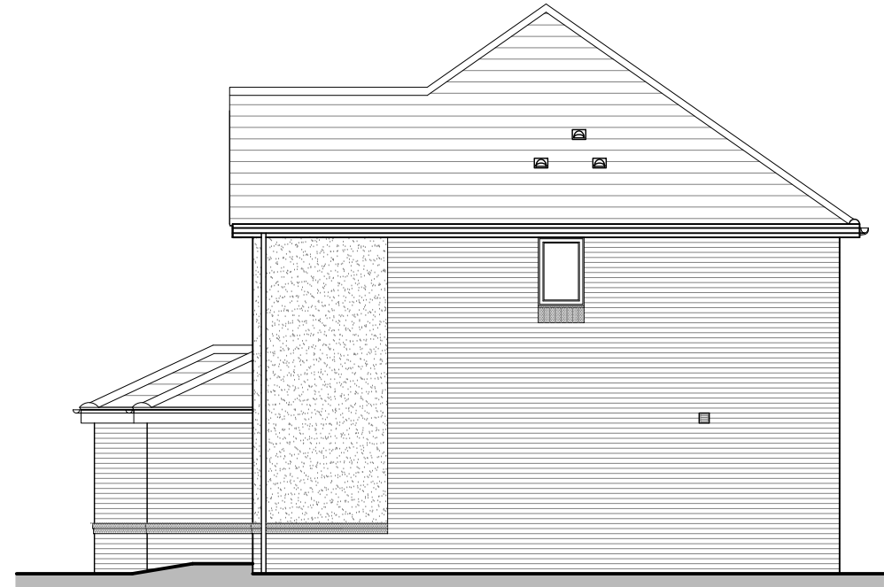
SIDE ELEVATION BRO.TF.2 (AS)
