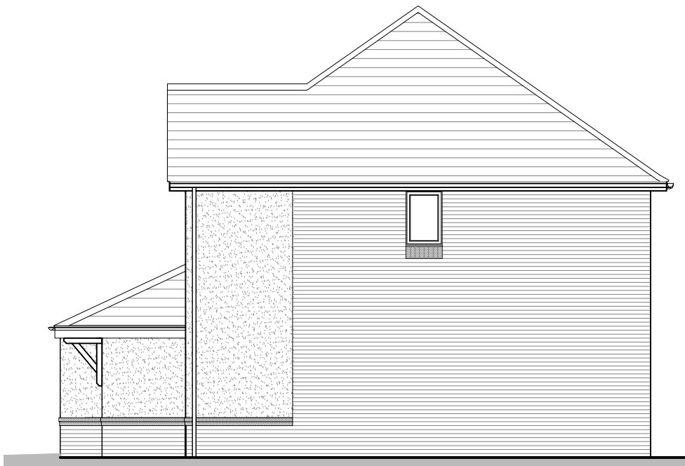
SIDE ELEVATION EVE.TF.2 (AS)
