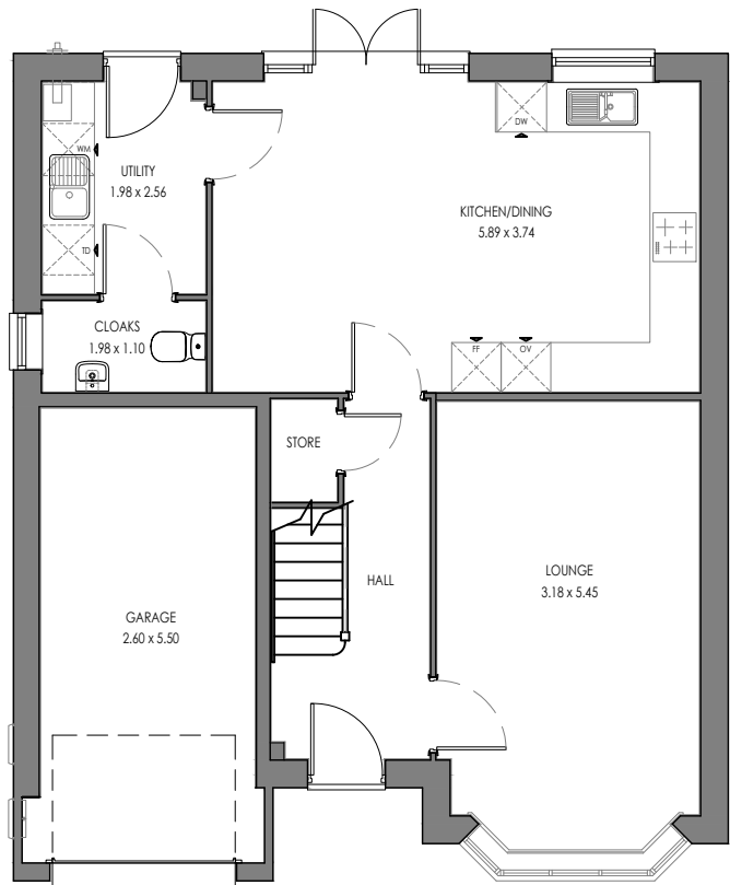
WEN.TF.2 (AS) GROUND FLOOR
