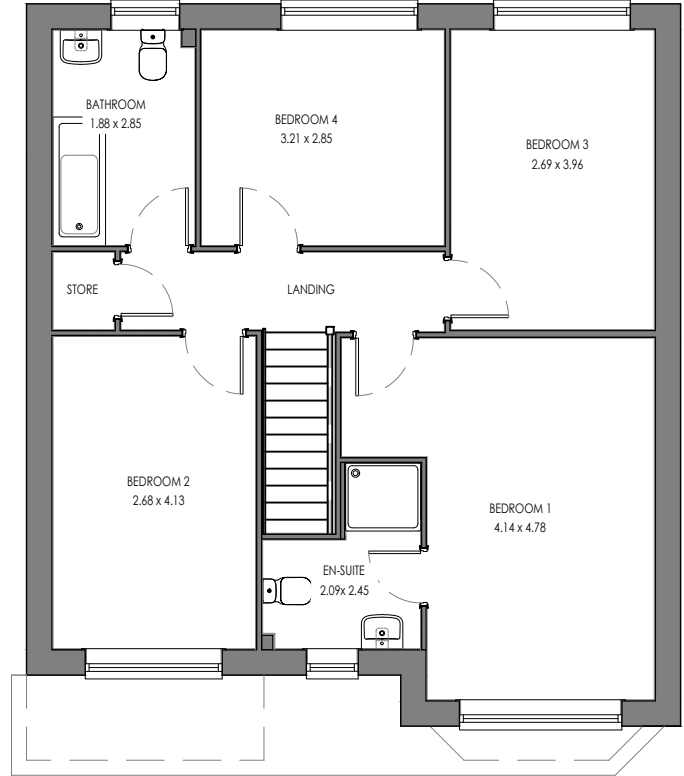
WEN.TF.2 (AS) FIRST FLOOR
