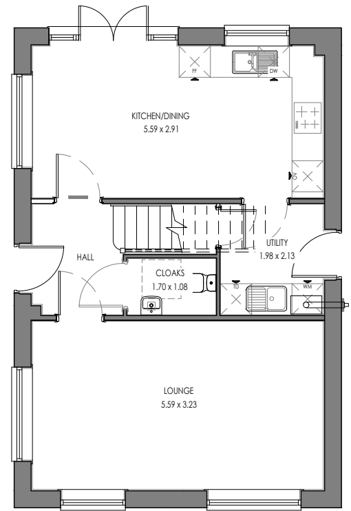
HEN.TF.2 (AS) GROUND FLOOR
