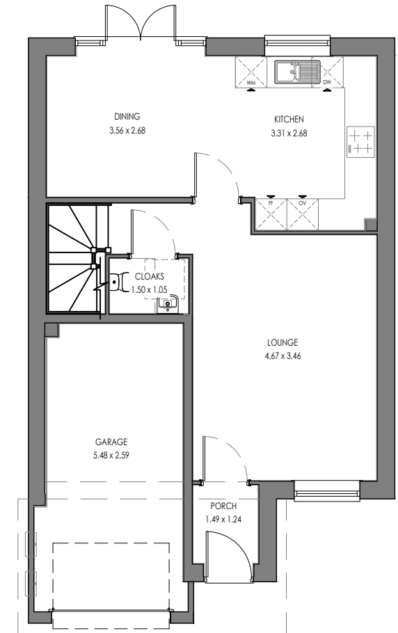
KIN.TF.1 (AS) GROUND FLOOR
