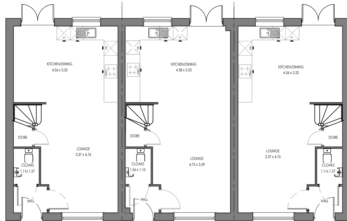
HIG.E.TF.1 (AS) GROUND FLOOR OPEN PLAN
