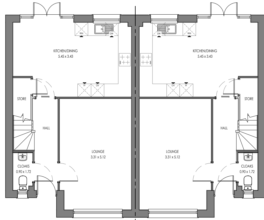
MAR.E.TF.2 (AS) GROUND FLOOR
