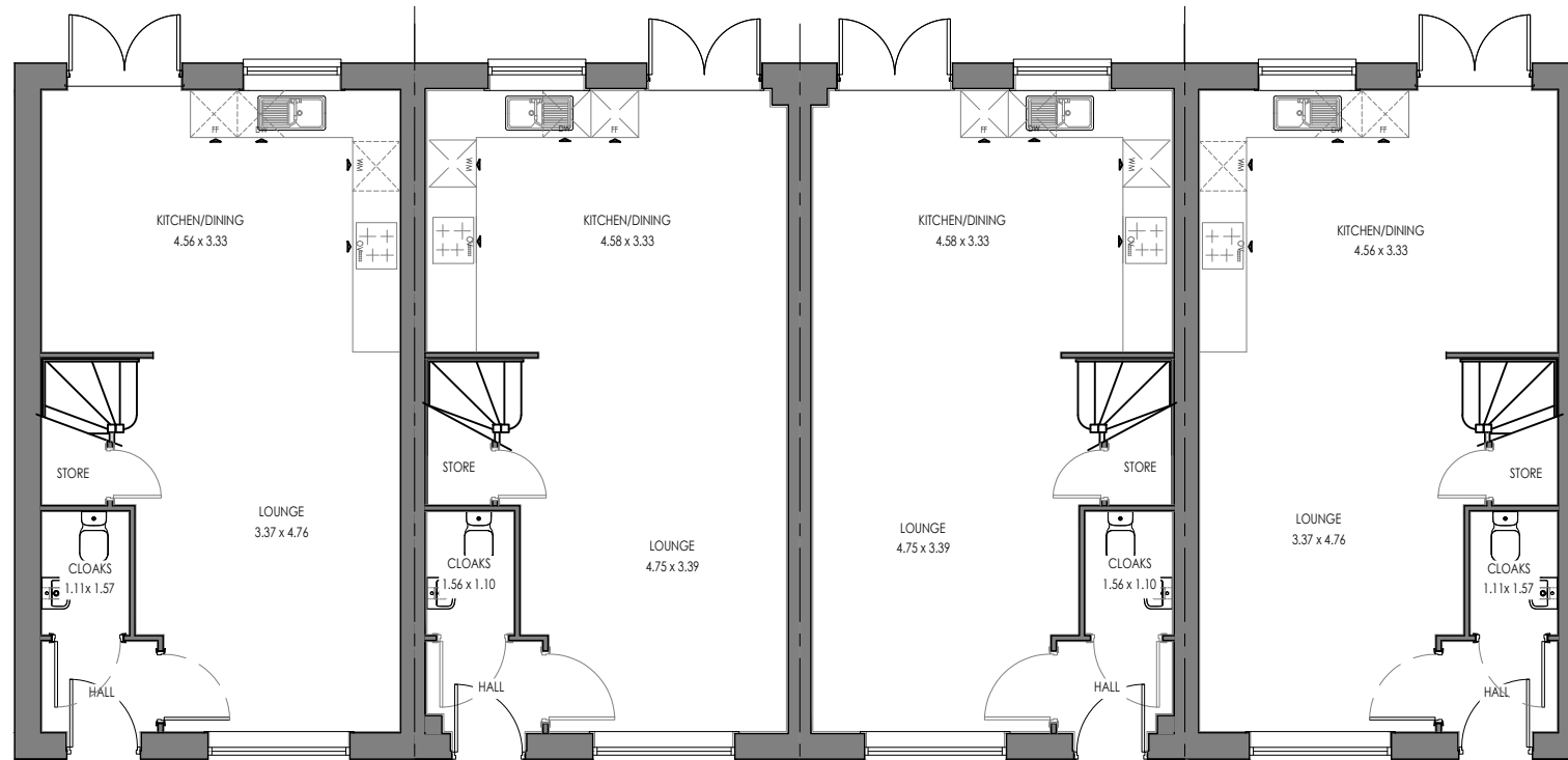
HIG.E.TF.1 (AS) GROUND FLOOR OPEN PLAN
