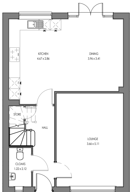
BUR.TF.2 (AS) GROUND FLOOR
