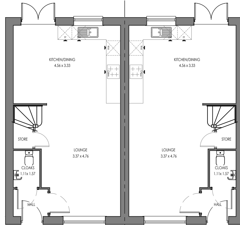
HIG.E.TF.1 (AS) GROUND FLOOR OPEN PLAN
