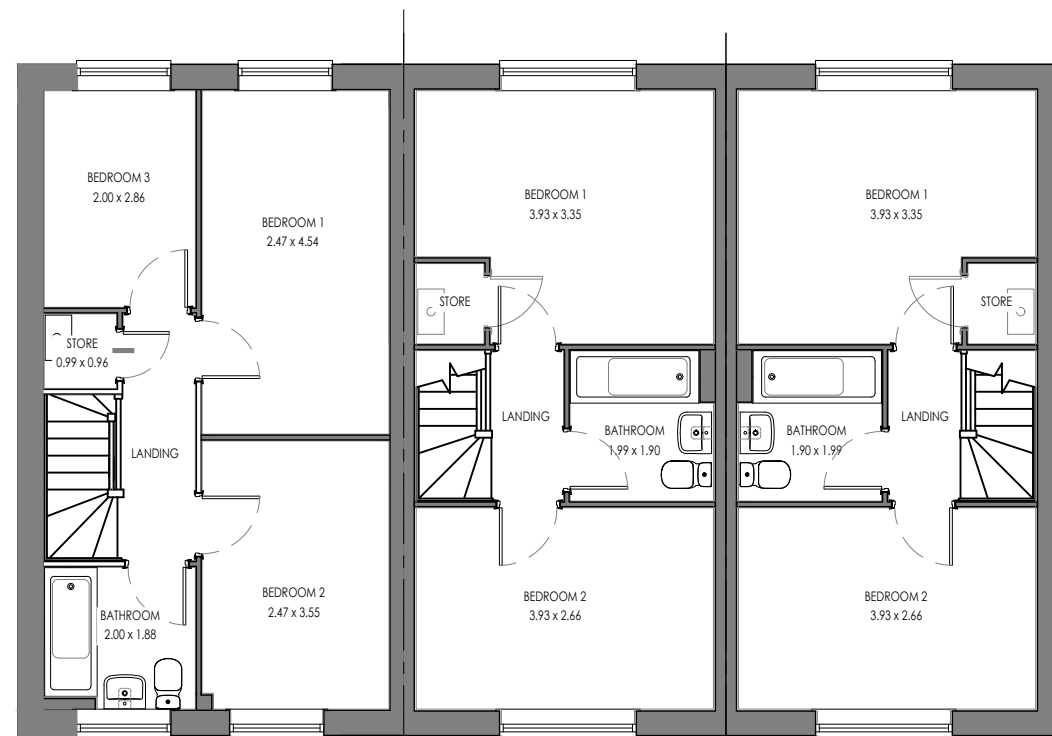
OAK.E.TF.1 (AS) FIRST FLOOR
