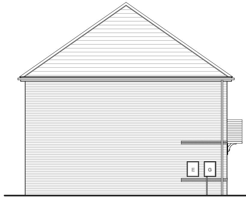
HIG.E.TF.1 (AS) SIDE ELEVATION
