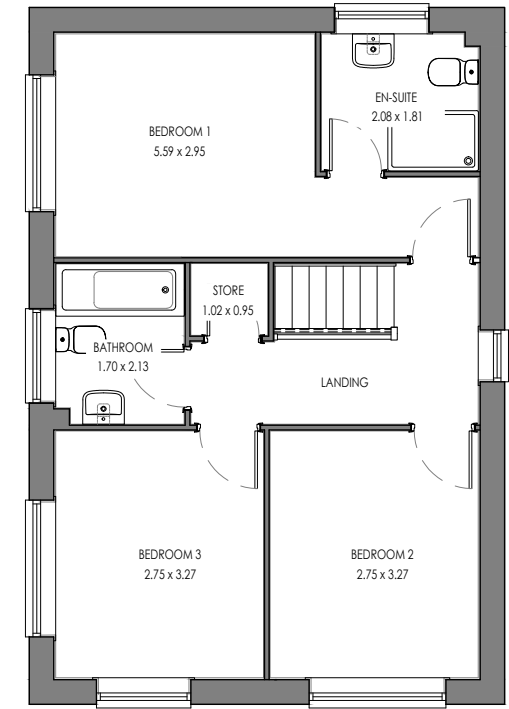
HEN.TF.2 (AS) FIRST FLOOR
