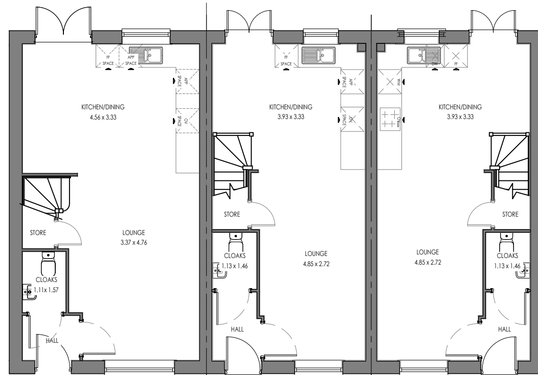
OAK.M.TF.1 (AS) GROUND FLOOR OPEN PLAN
