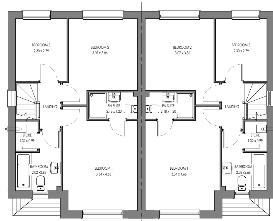
MAR.E.TF.2 (AS) FIRST FLOOR
