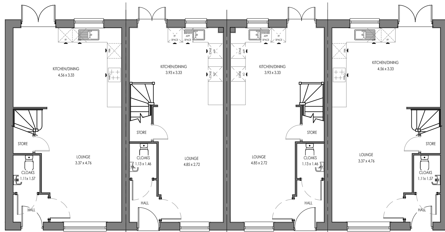
HIG.E.TF.1 (AS) GROUND FLOOR OPEN PLAN
