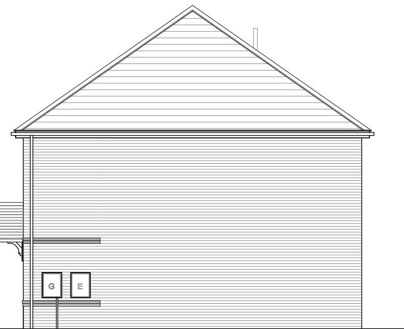
HIG.E.TF.1 (AS) SIDE ELEVATION
