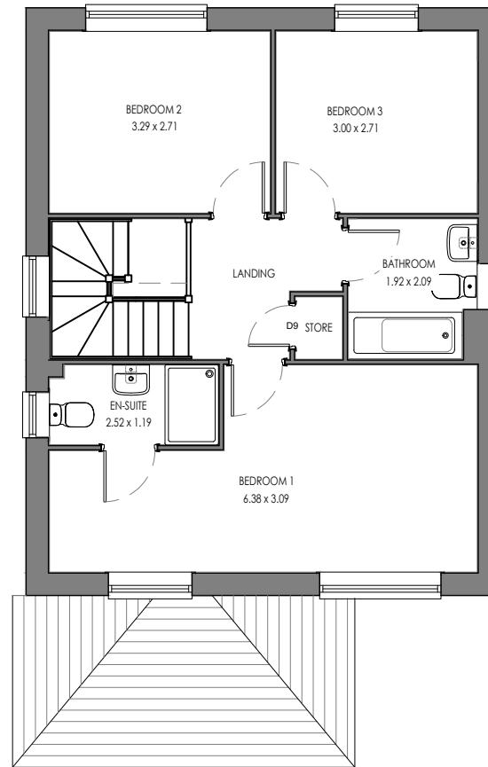
STR.TF.2 (AS) FIRST FLOOR
