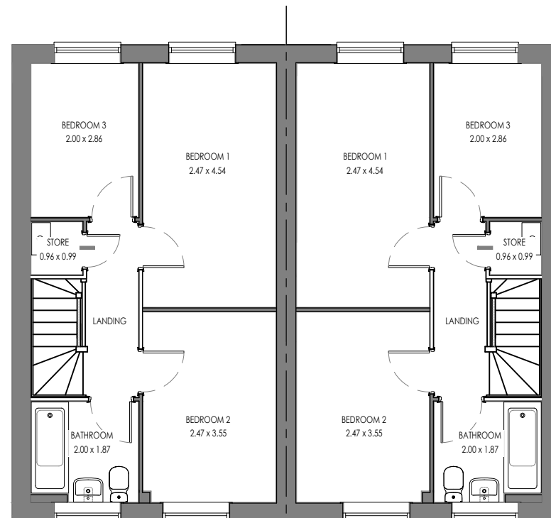
HIG.E.TF.1 (AS) FIRST FLOOR
