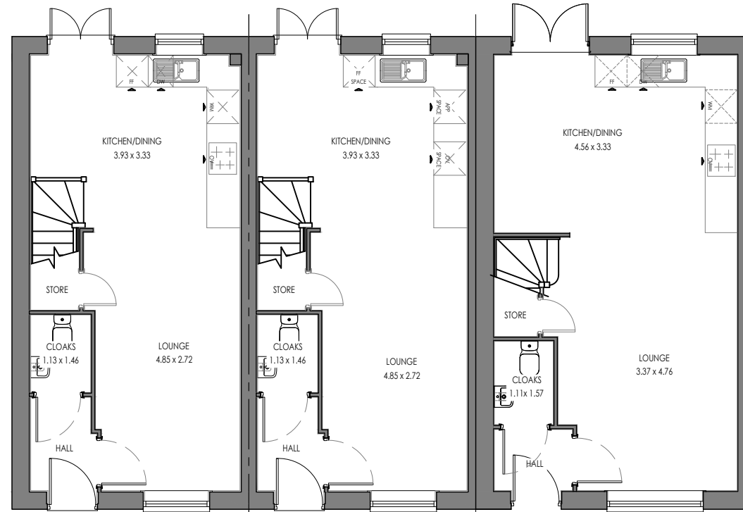
OAK.E.TF.1 (AS) GROUND FLOOR OPEN PLAN
