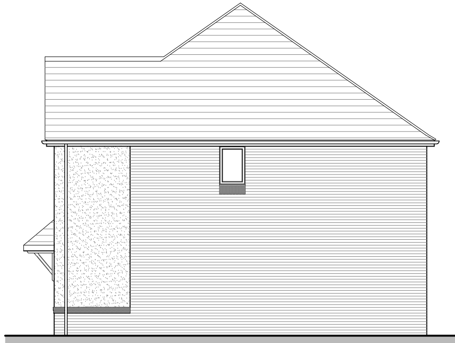
BUR.TF.2 (AS) SIDE ELEVATION
