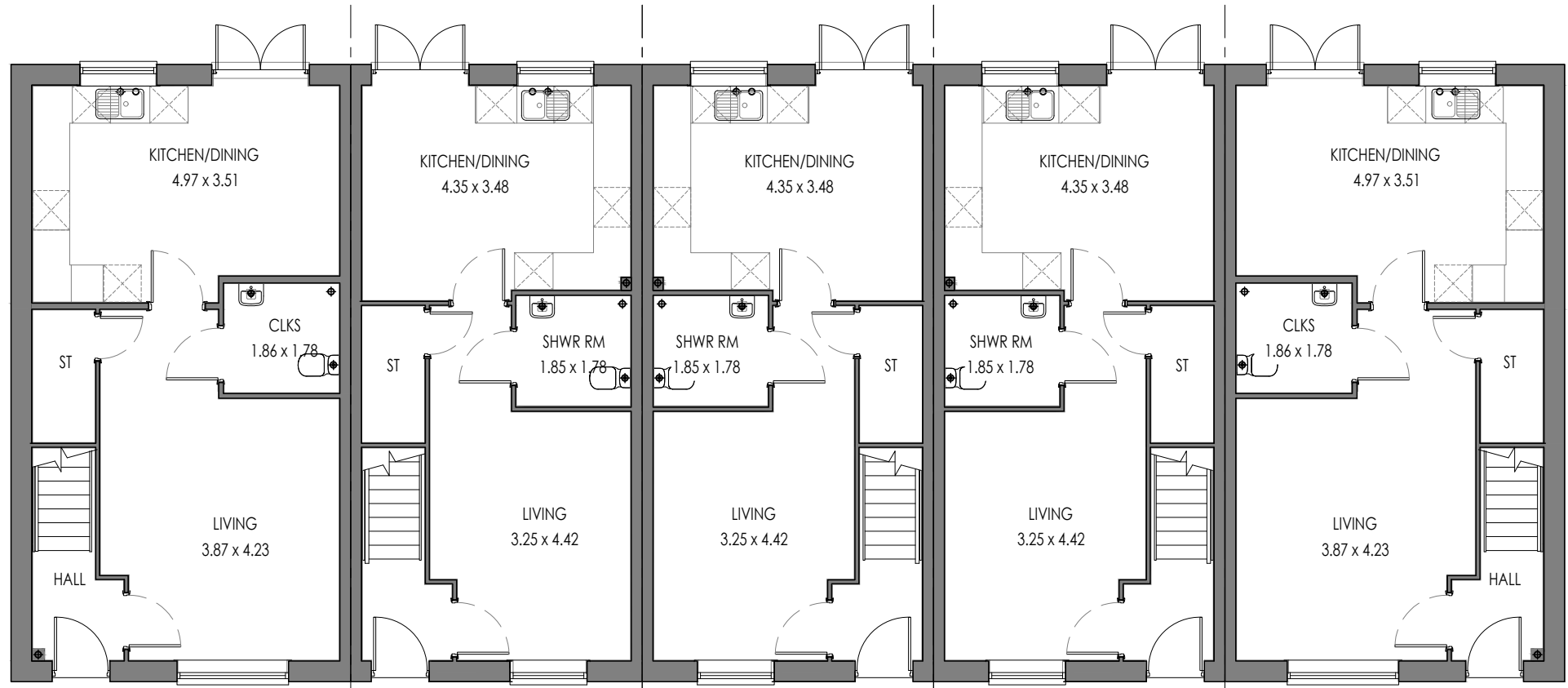
5P3B END (AS) GROUND FLOOR 4P2B MID (AS) GROUND FLOOR 4P2B MID (OPP) GROUND FLOOR 4P2B MID (OPP) GROUND FLOOR 5P3B END (OPP) GROUND FLOOR
