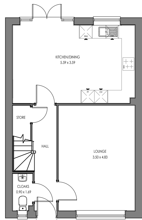
OXF.TF.2 (AS) GROUND FLOOR
