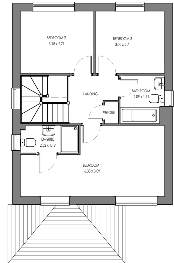
KIN.TF.1 (AS) FIRST FLOOR
