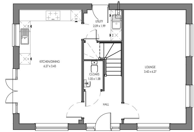
BEW.TF.1 (AS) GROUND FLOOR
