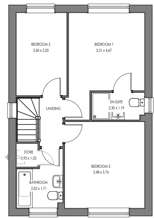
OXF.TF.2 (AS) FIRST FLOOR
