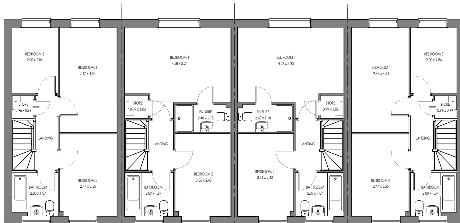
HIG.E.TF.1 (AS) FIRST FLOOR
