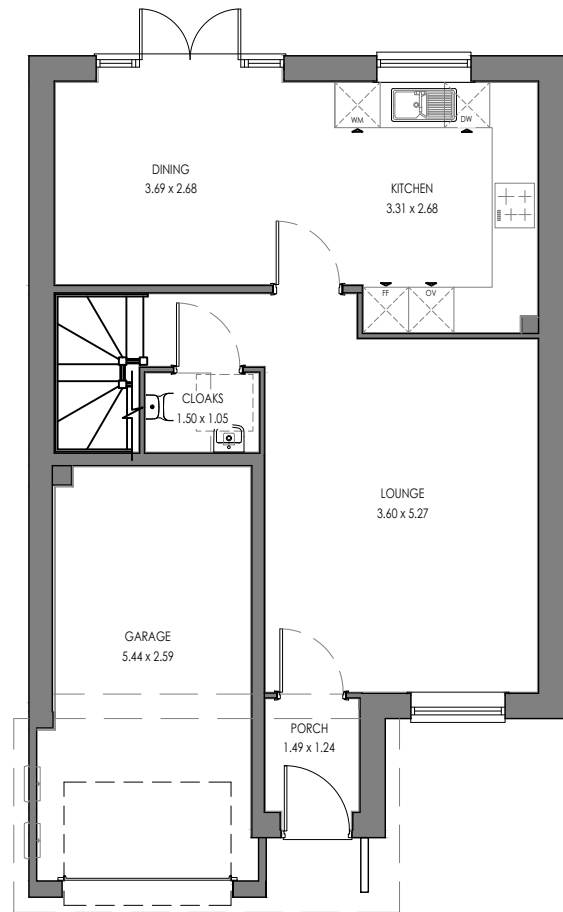
STR.TF.2 (AS) GROUND FLOOR
