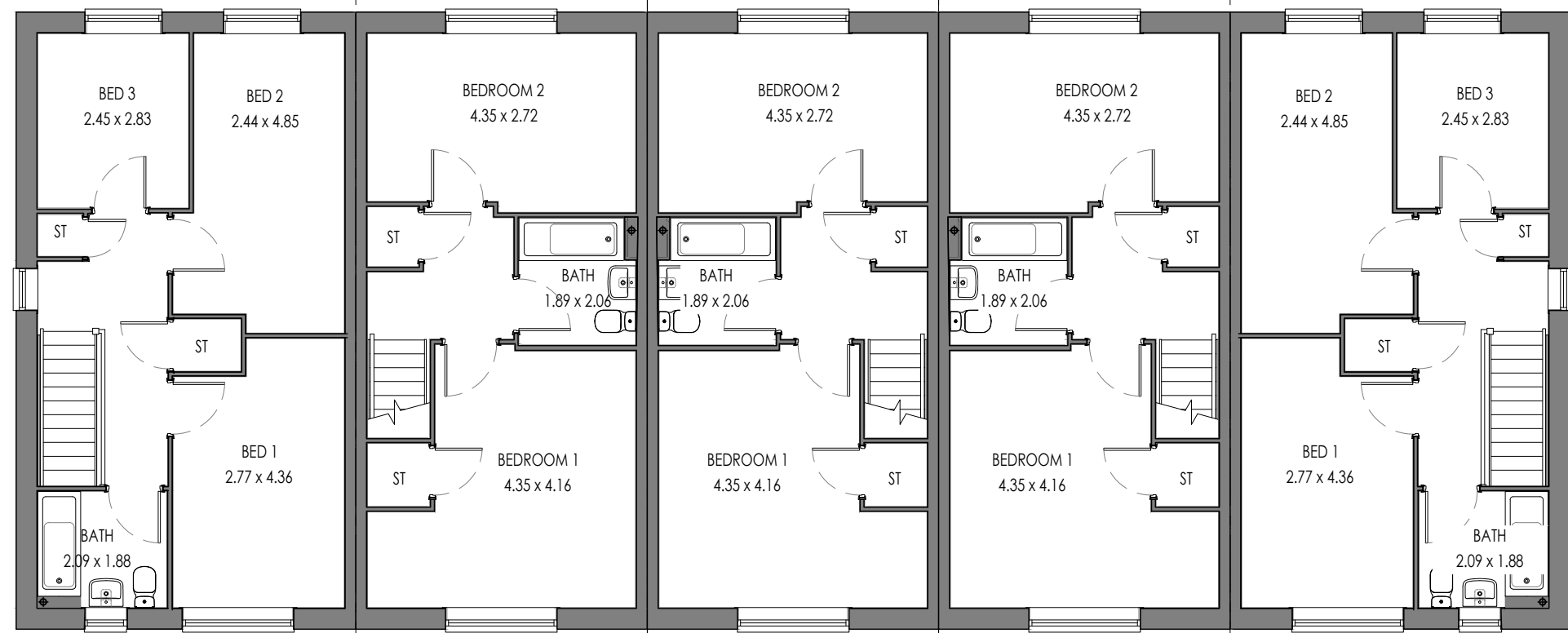
5P3B END (AS) FIRST FLOOR 4P2B MID (AS) FIRST FLOOR 4P2B MID (OPP) FIRST FLOOR 4P2B MID (OPP) FIRST FLOOR 5P3B END (OPP) FIRST FLOOR
