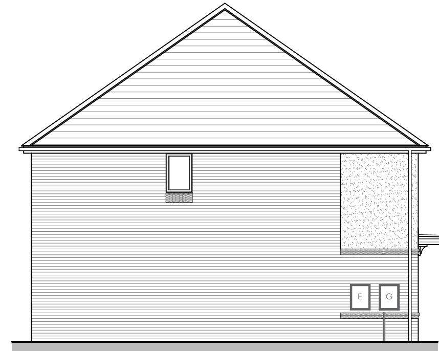
6P4B END (AS) SIDE ELEVATION
