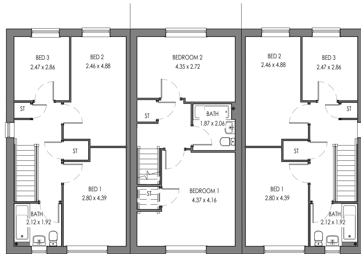
5P3B END (AS) FIRST FLOOR
