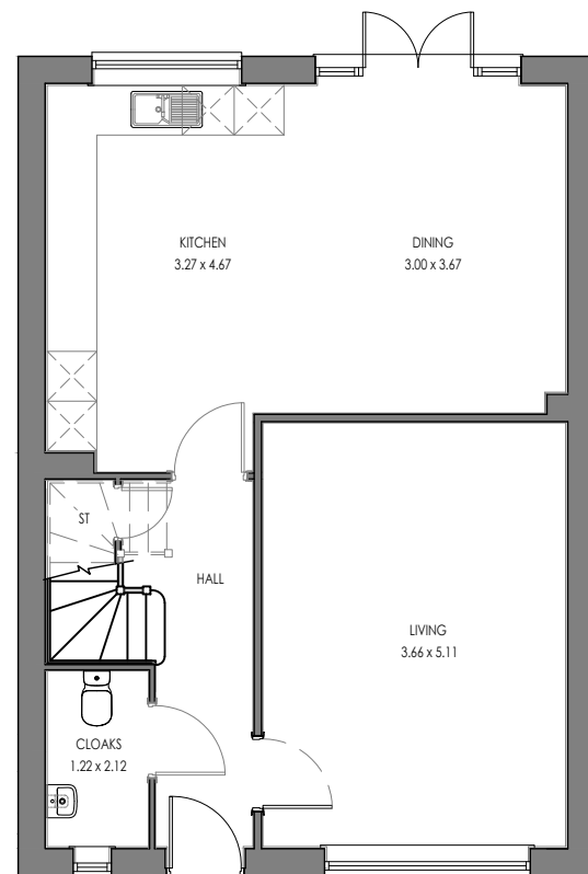
BURLINGTON (AS) GROUND FLOOR
