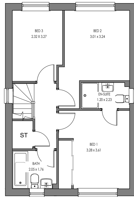
HARTFORD (AS) FIRST FLOOR
