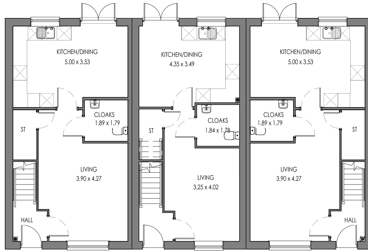
4P2B MID (AS) GROUND FLOOR
