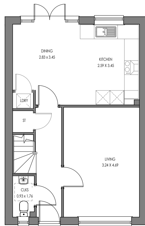
HARTFORD (AS) GROUND FLOOR
