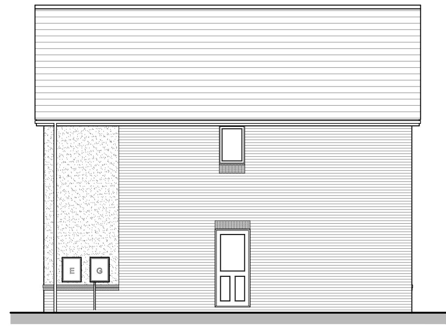
BEWLEY (AS) REAR ELEVATION
