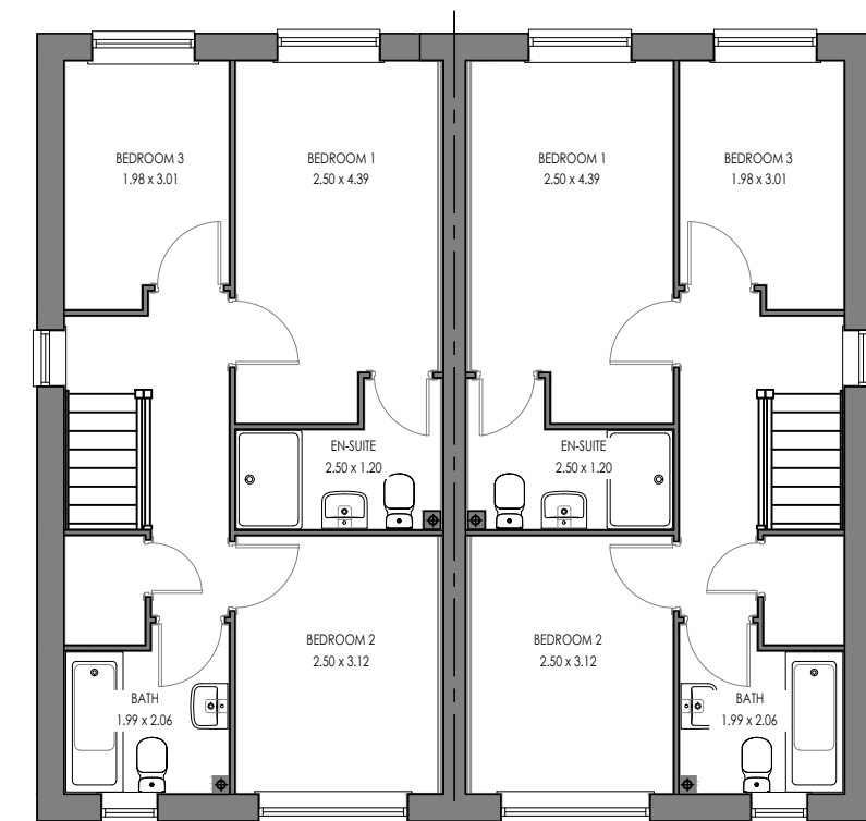
HUXLEY (AS) FIRST FLOOR
