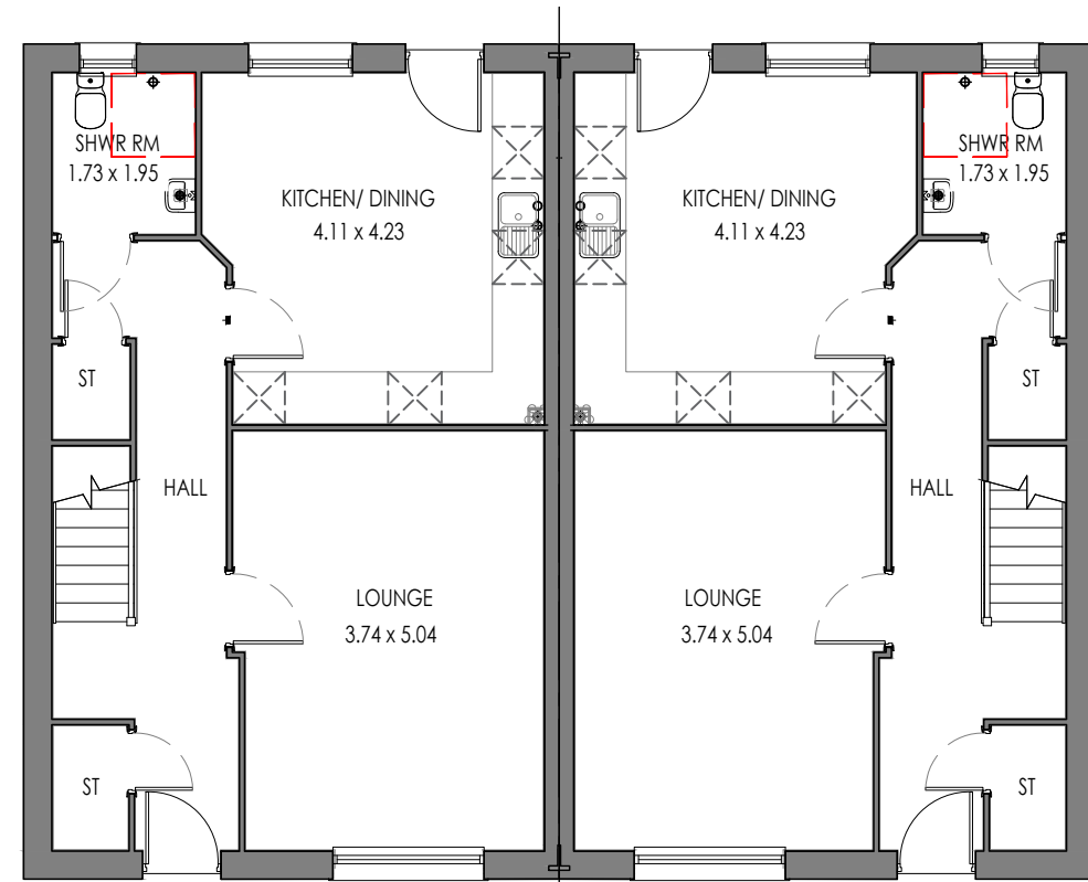
6P4B END (AS) GROUND FLOOR
