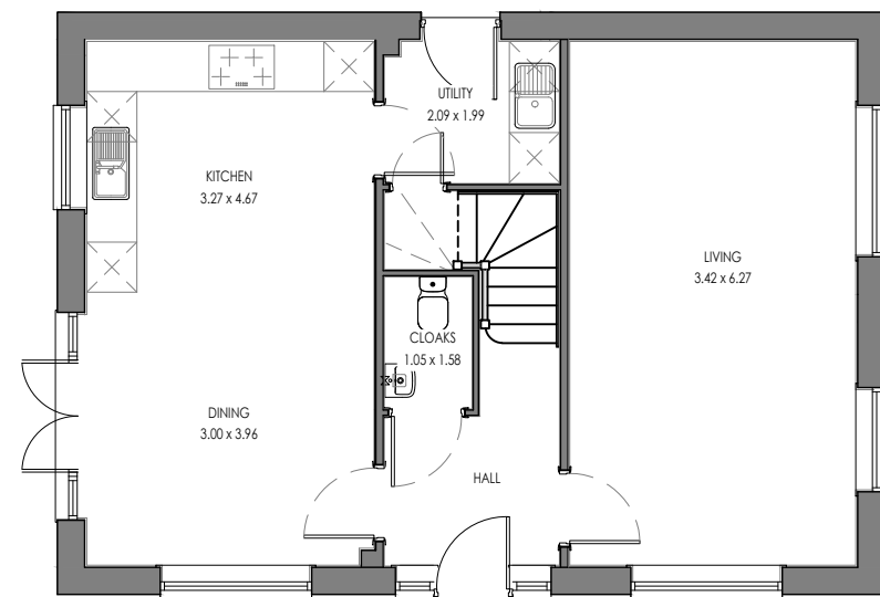
BEWLEY (AS) GROUND FLOOR
