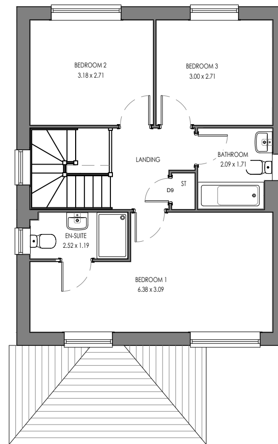
KINGSLEY (AS) FIRST FLOOR
