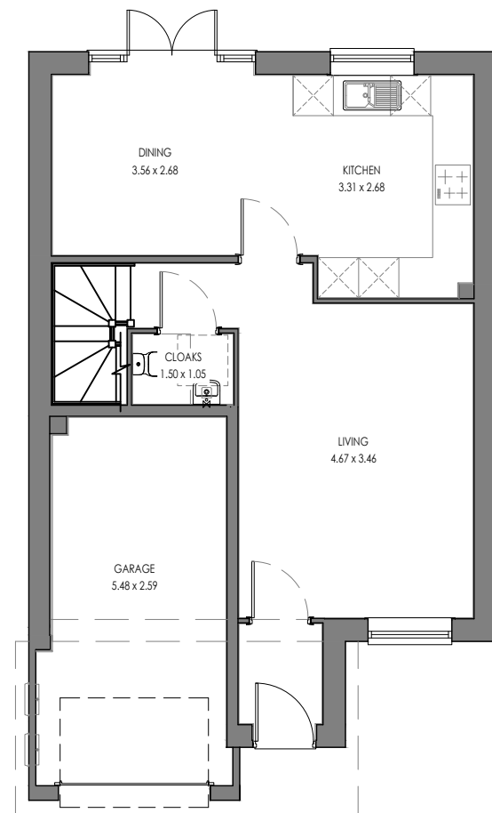
KINGSLEY (AS) GROUND FLOOR
