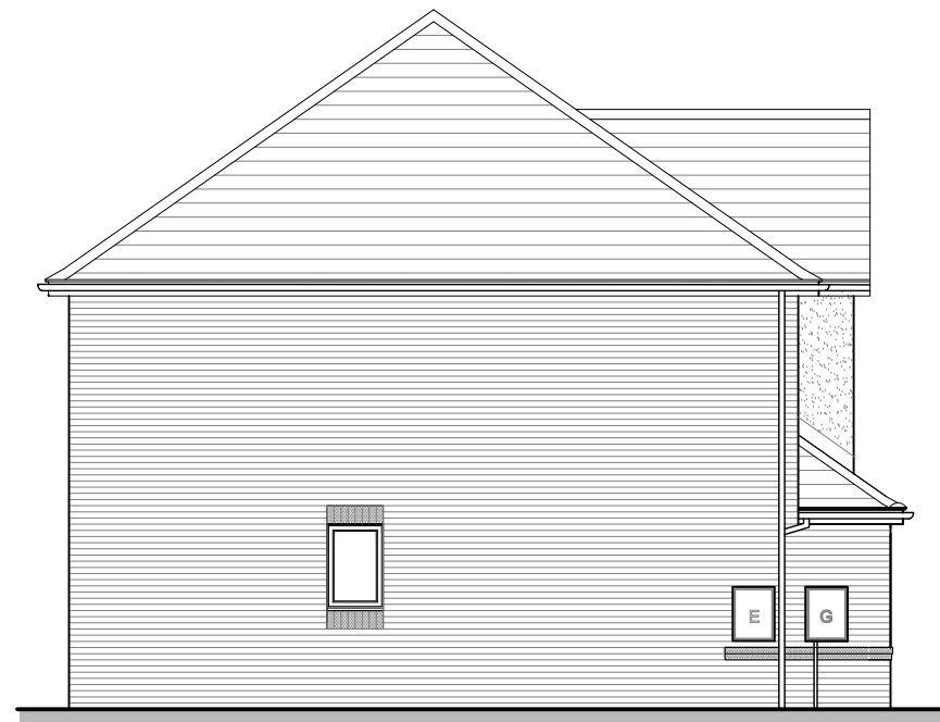
WENTWORTH (AS) SIDE ELEVATION
