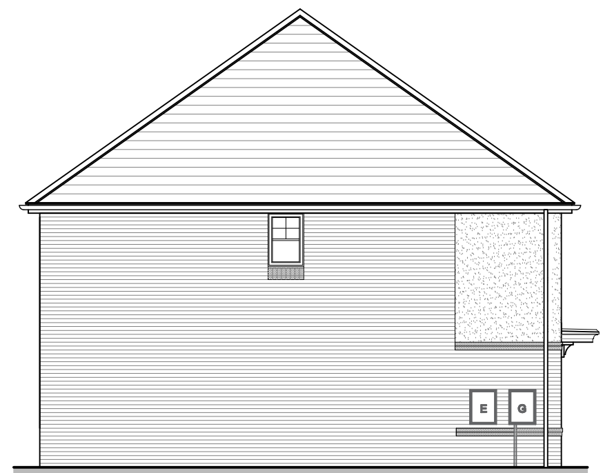
4P2B END (AS) SIDE ELEVATION
