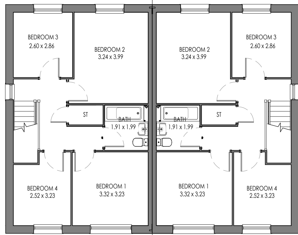
6P4B END (AS) FIRST FLOOR
