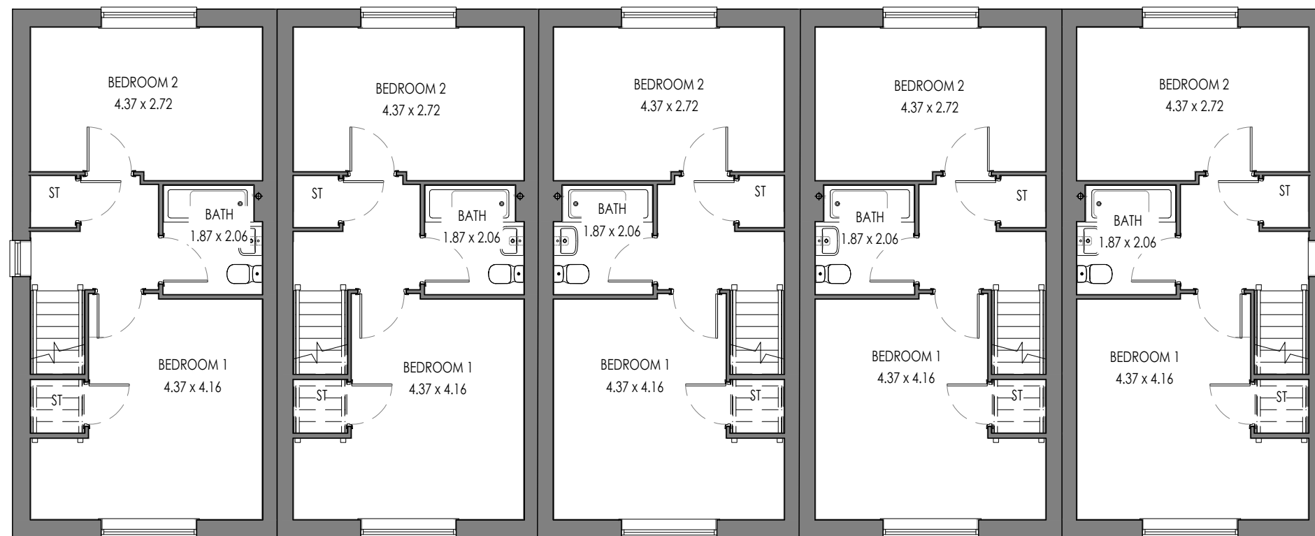
4P2B MID (AS) FIRST FLOOR
