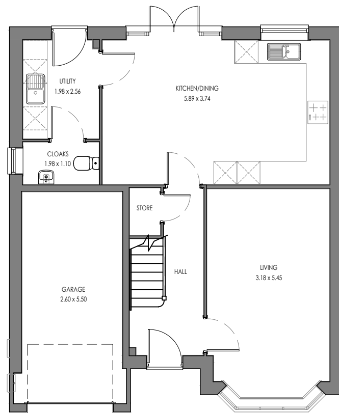
WENTWORTH (AS) GROUND FLOOR
