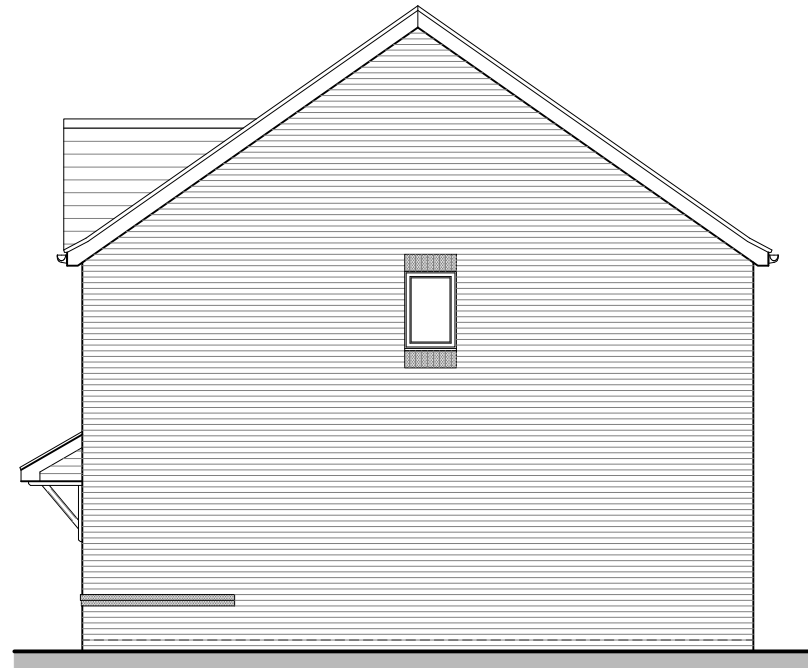
HARTFORD (AS) SIDE ELEVATION
