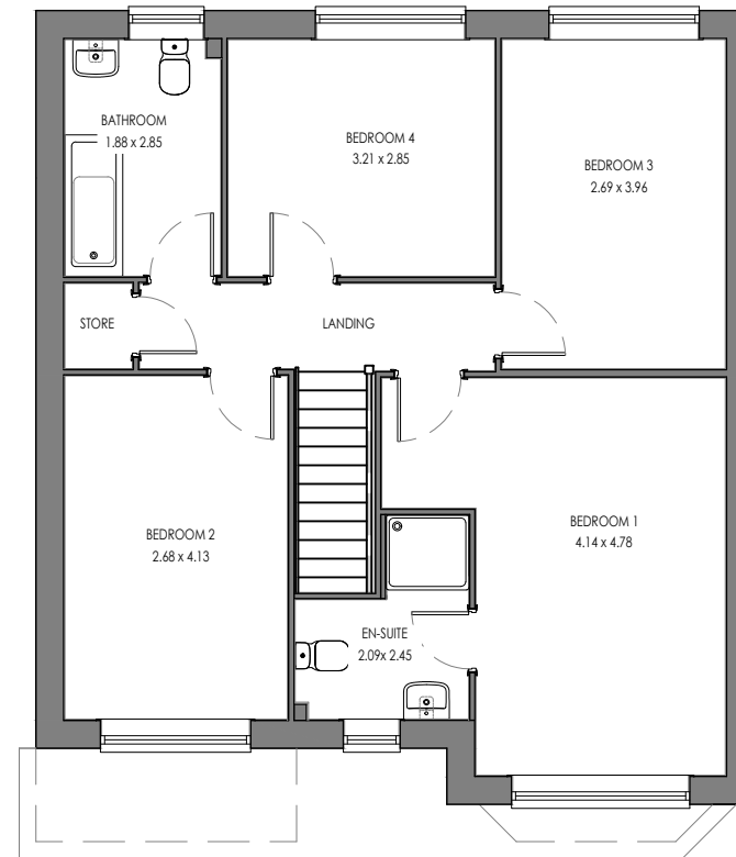
WENTWORTH (AS) FIRST FLOOR
