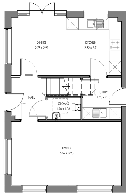
HENLEY (AS) GROUND FLOOR
