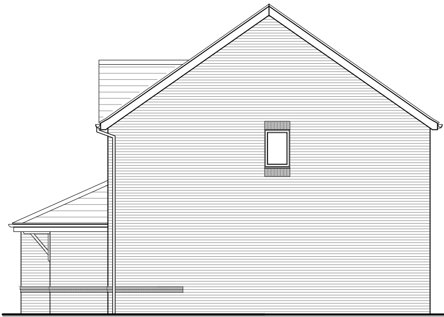
KINGSLEY (AS) SIDE ELEVATION
