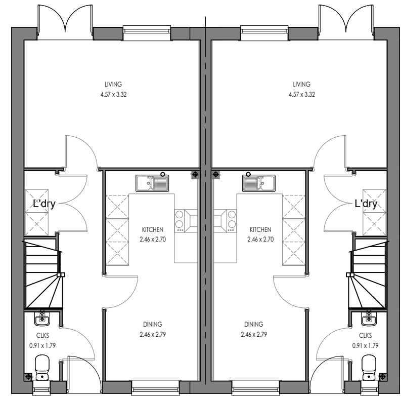
HUXLEY (AS) GROUND FLOOR
