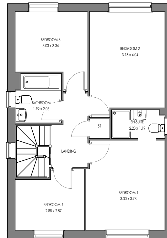
BURLINGTON (AS) FIRST FLOOR
