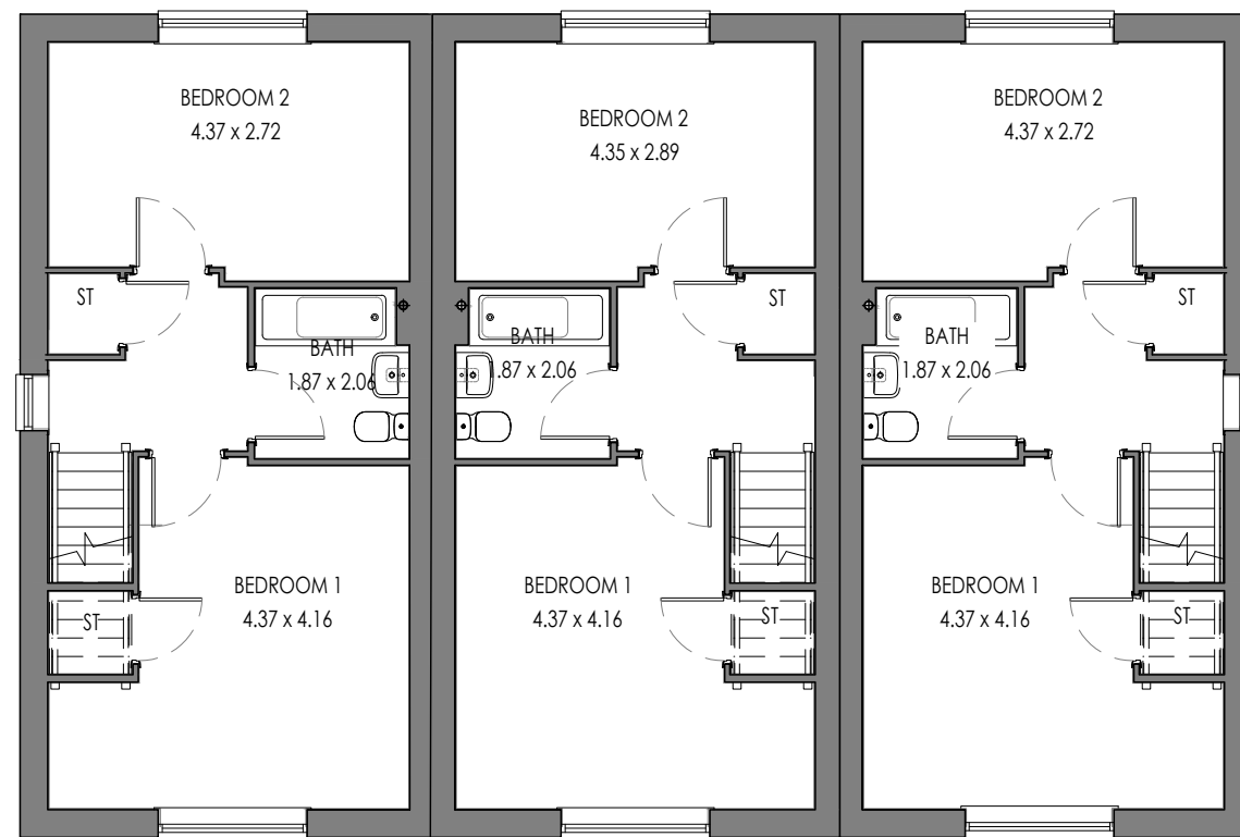
4P2B END (AS) FIRST FLOOR
