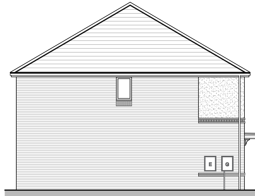
4P2B (AS) SIDE ELEVATION
