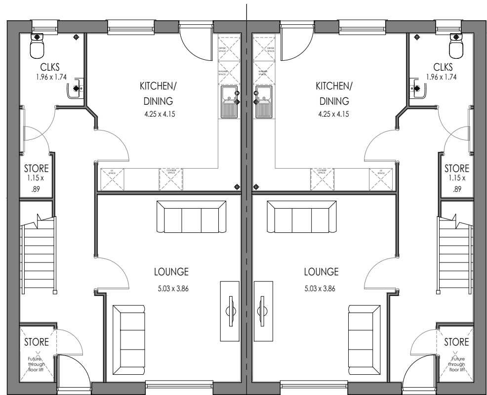
6P4B OPP GROUND FLOOR
