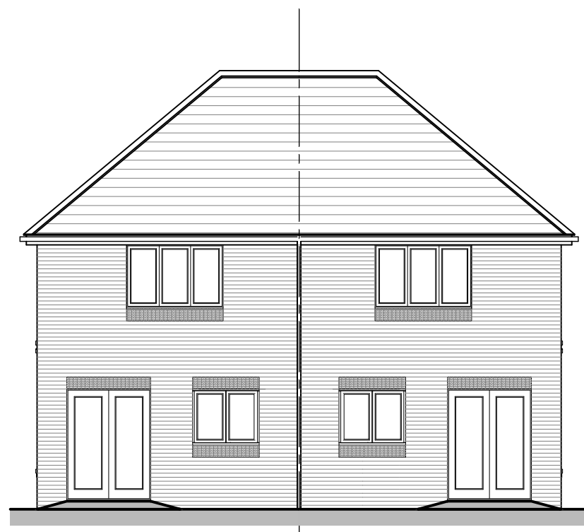
4P2B (OPP) REAR ELEVATION
