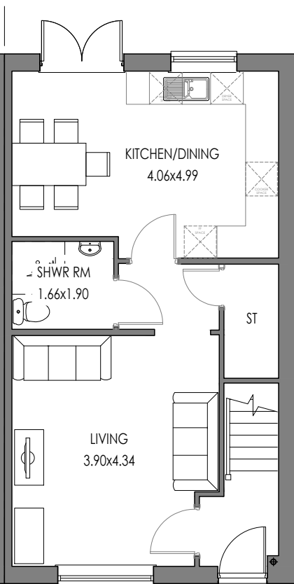
GROUND FLOOR 5P3B (OPP)
