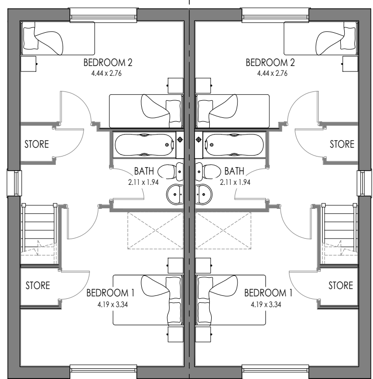
4P2B END AS FIRST FLOOR
