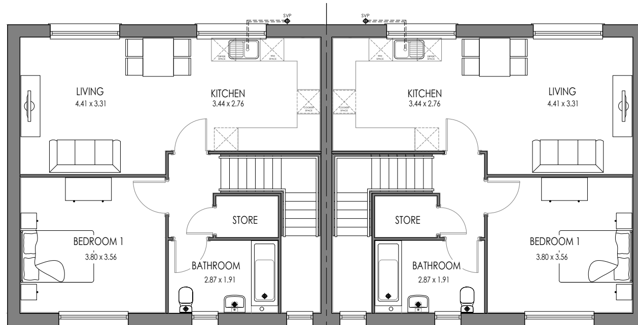
2P1B AS FIRST FLOOR
