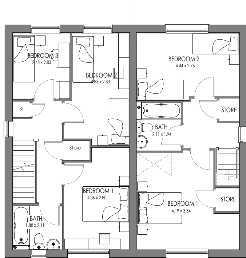
5P3B END AS FIRST FLOOR
