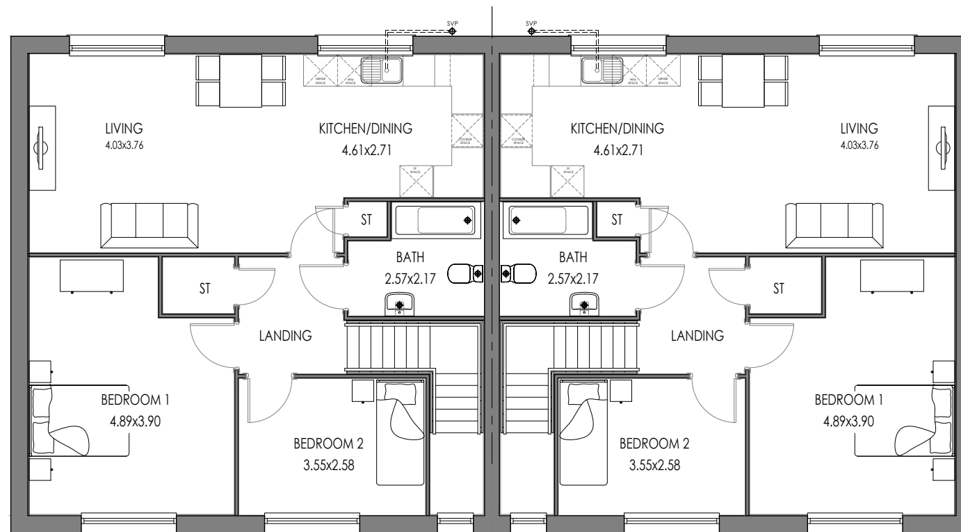
3P2B AS FIRST FLOOR
