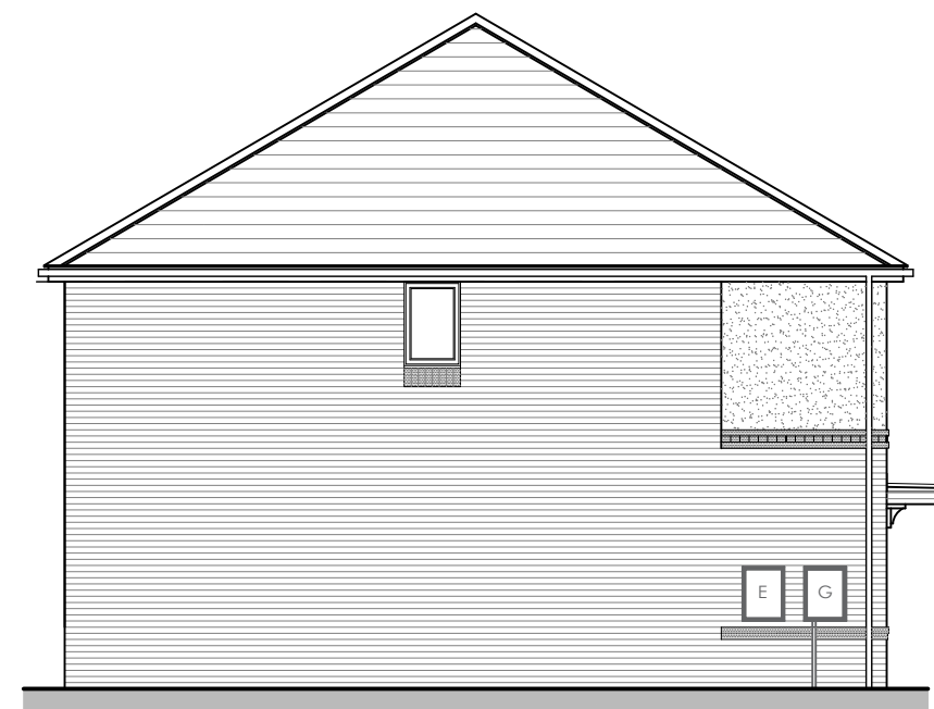
5P3B (AS) SIDE ELEVATION
