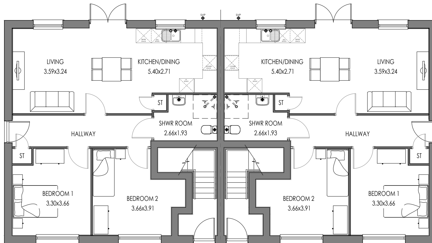
3P2B AS GROUND FLOOR
