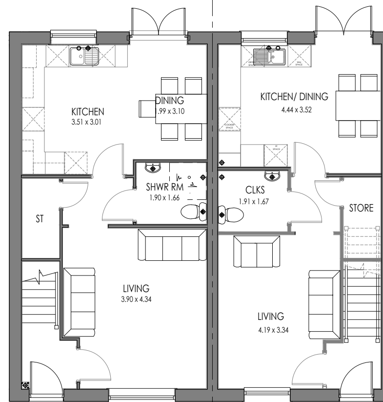
5P3B END AS GROUND FLOOR
