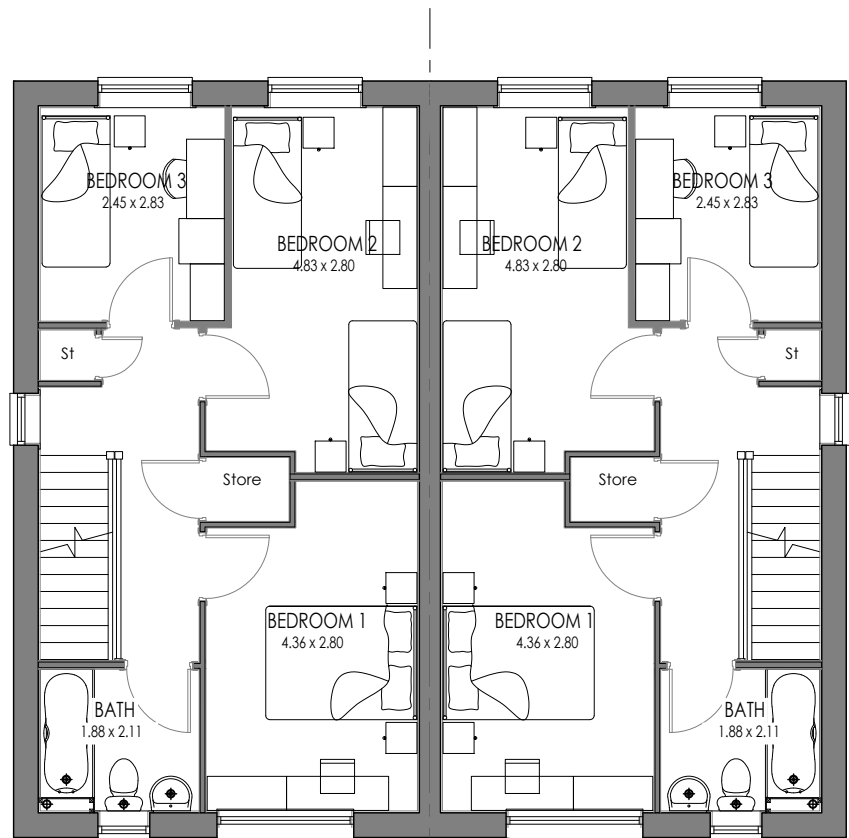
5P3B END AS FIRST FLOOR
