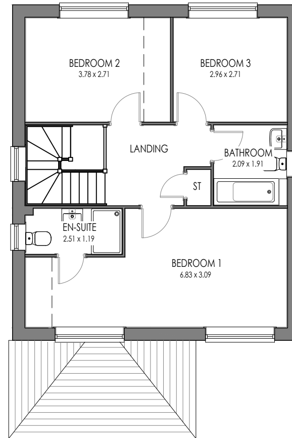
EVESHAM (AS) FIRST FLOOR
