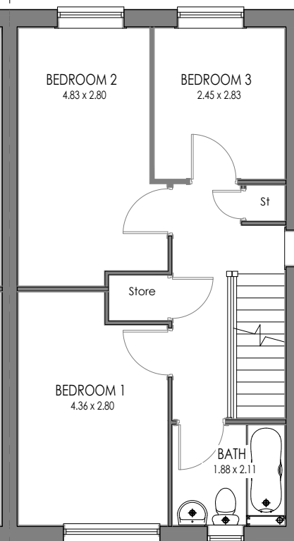
5P3B END (OPP) FIRST FLOOR
