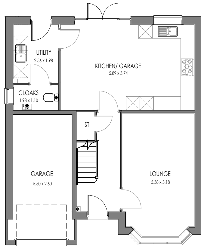
WENTWORTH 3 (AS) GROUND FLOOR
