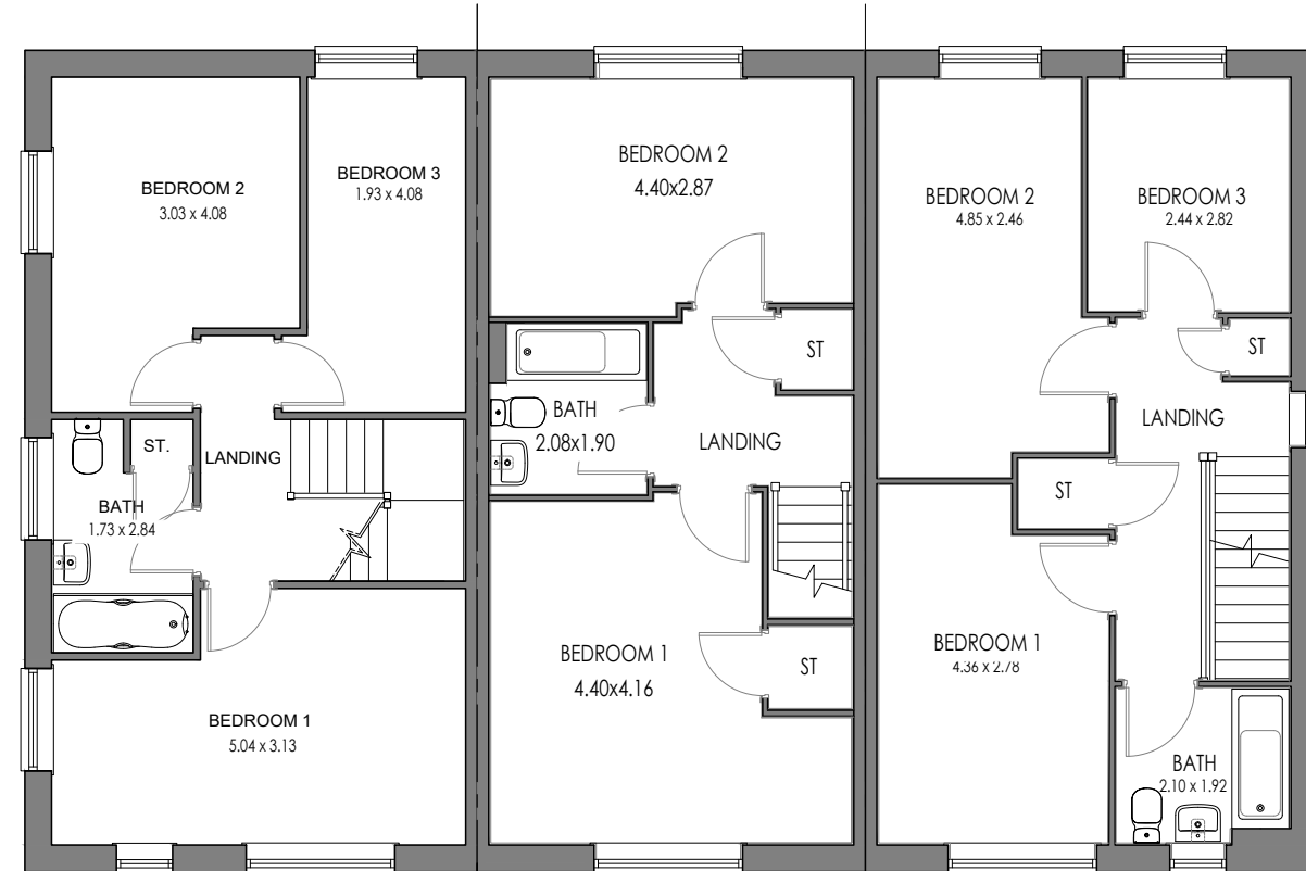
5P3B CORNER (AS) FIRST FLOOR
