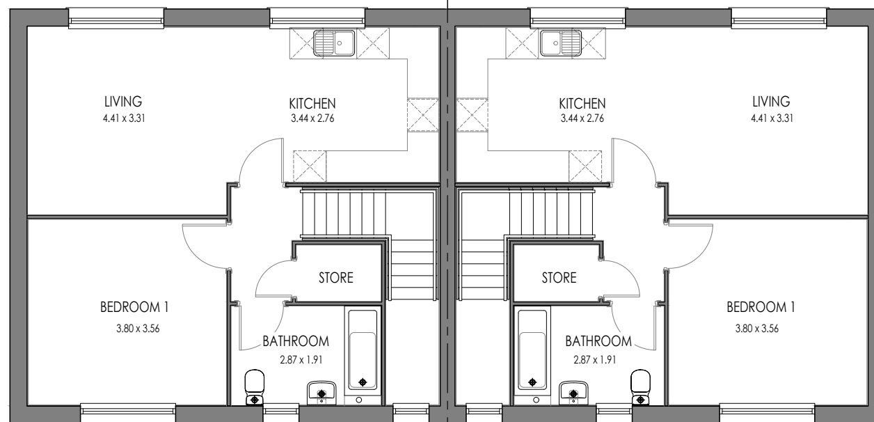
2P1B (AS) FIRST FLOOR
