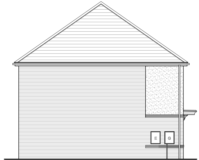
WARWICK (AS) SIDE ELEVATION
