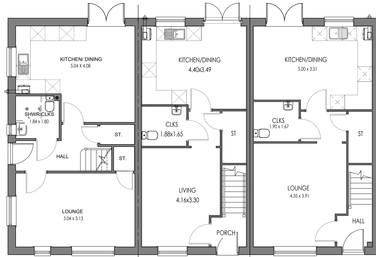
5P3B CORNER (AS) GROUND FLOOR
