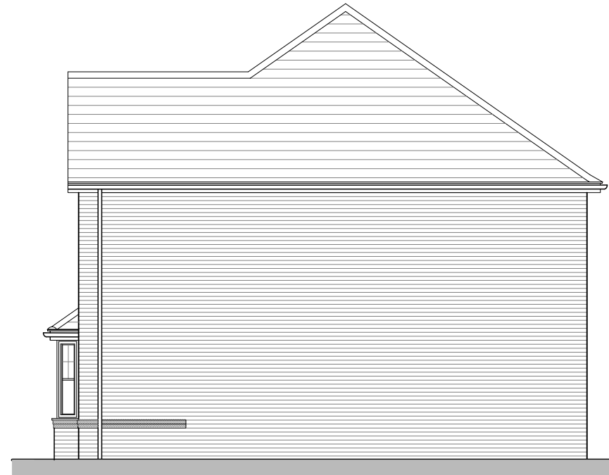
WENTWORTH 3 (AS) SIDE ELEVATION
