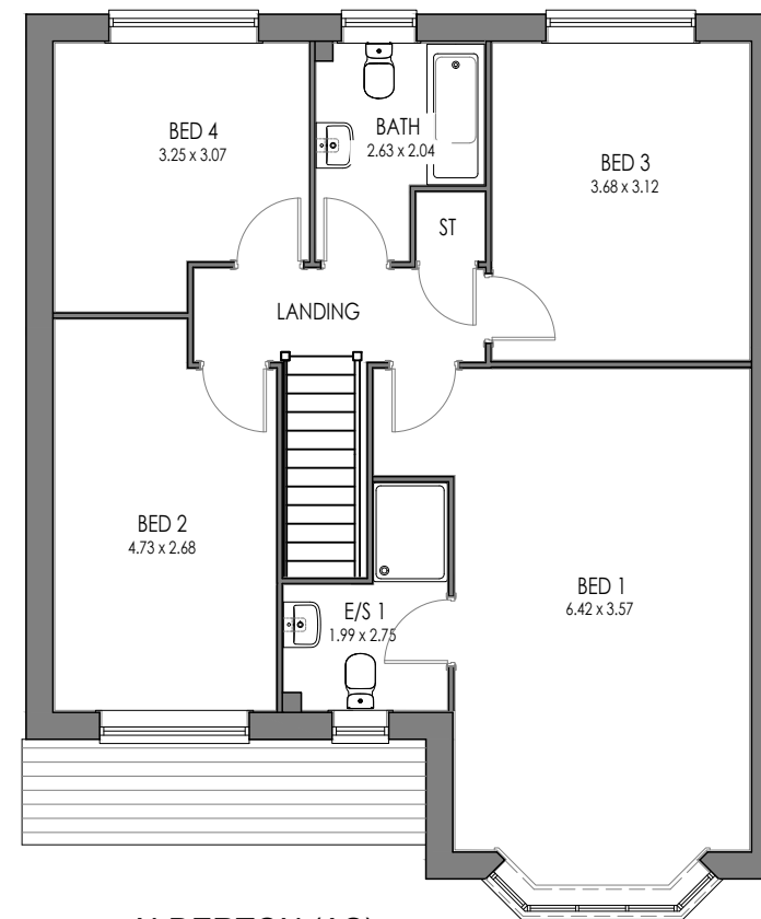
ALDERTON (AS) FIRST FLOOR
