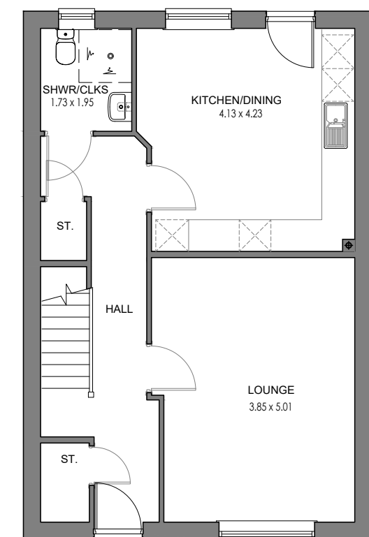
6P4B (AS) GROUND FLOOR
