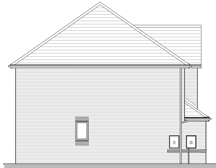
WENTWORTH 3 (AS) SIDE ELEVATION
