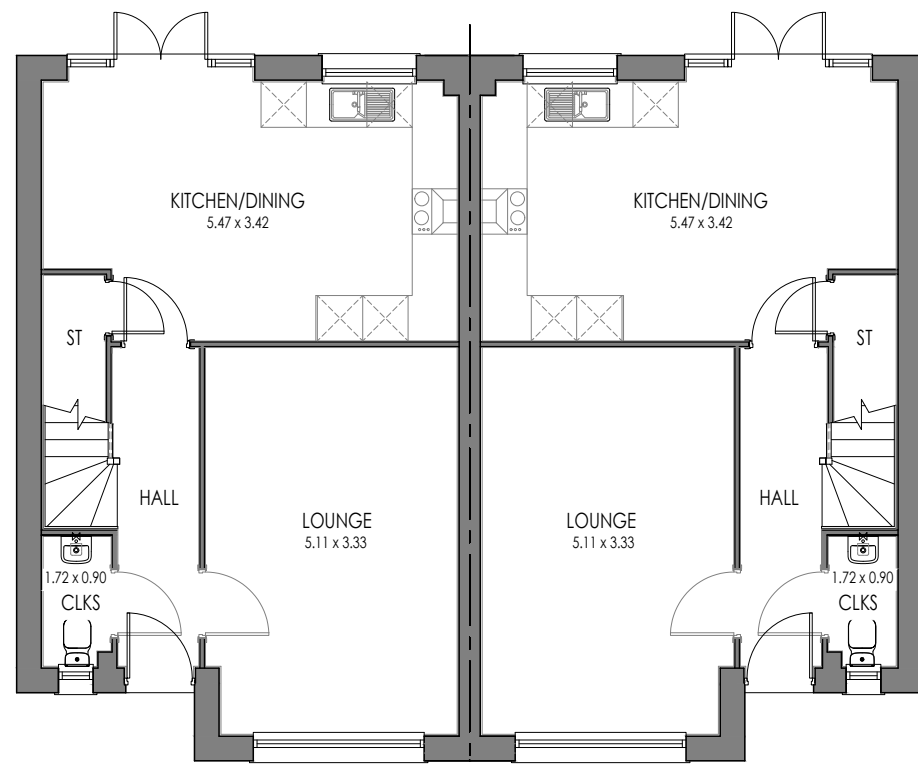
MARLOW SEMI (AS) GROUND FLOOR
