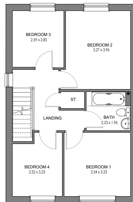
6P4B (AS) FIRST FLOOR
