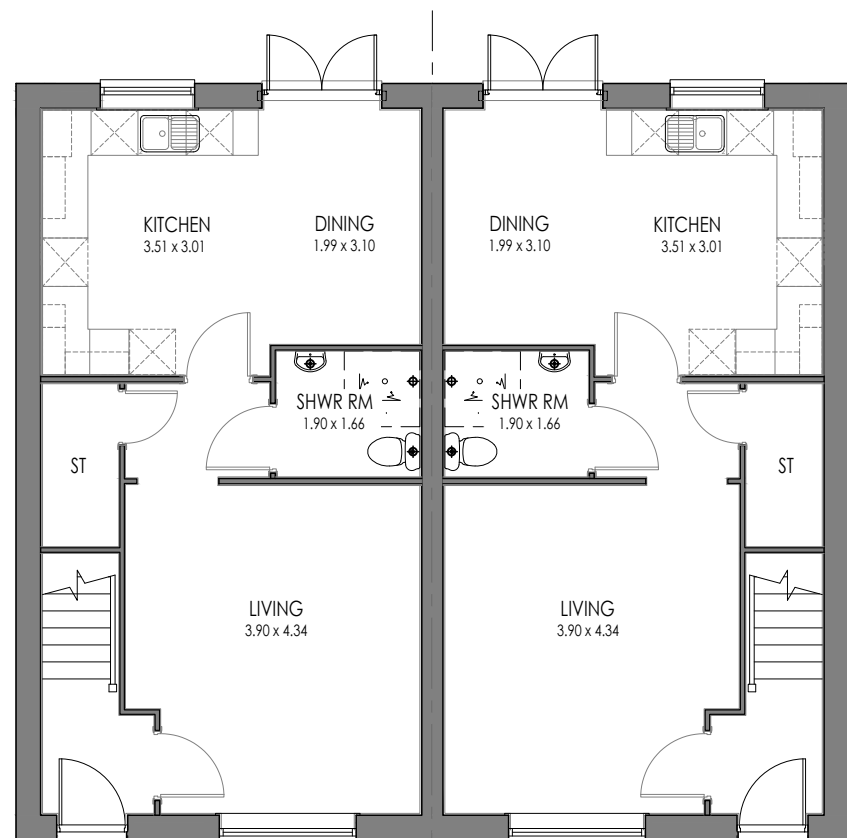
5P3B END (AS) GROUND FLOOR
