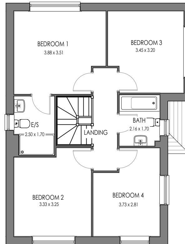
HEATHERINGTON (AS) FIRST FLOOR
