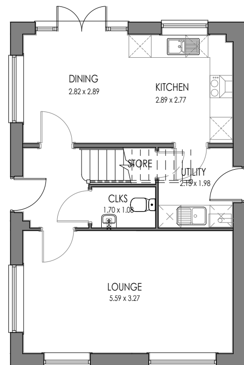
HENLEY (AS) GROUND FLOOR
