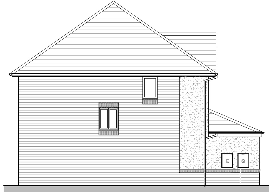
EVESHAM (AS) SIDE ELEVATION
