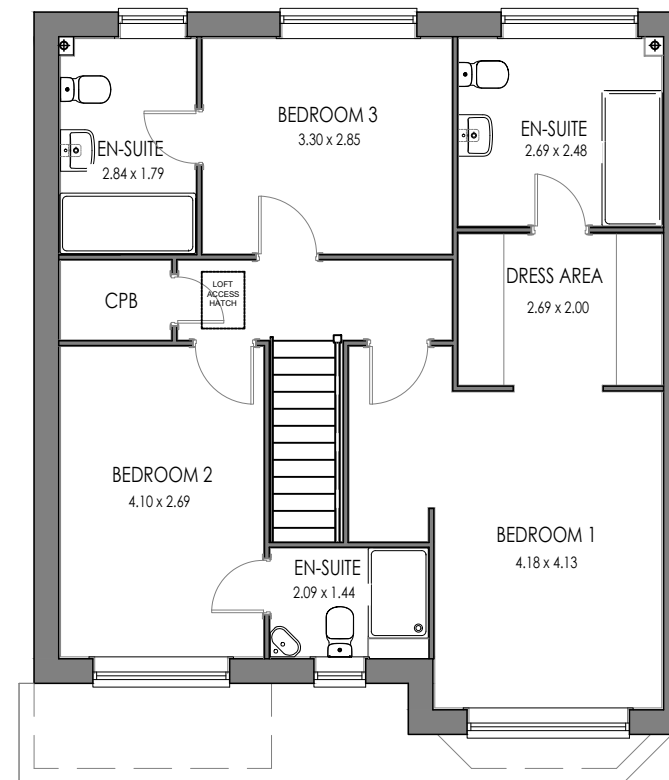
WENTWORTH 3 (AS) FIRST FLOOR
