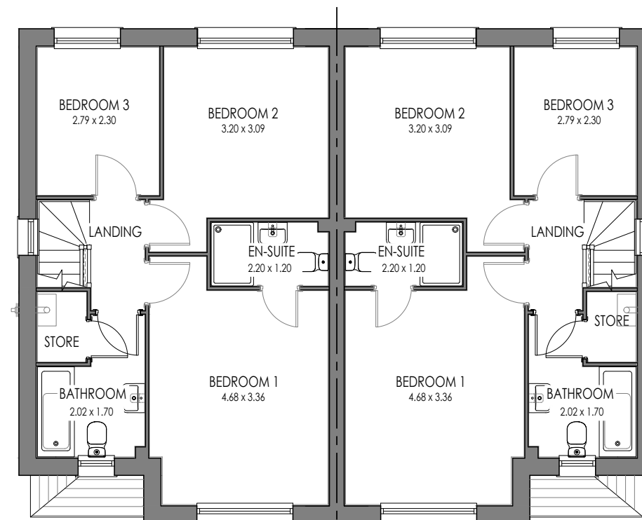
MARLOW SEMI (AS) FIRST FLOOR
