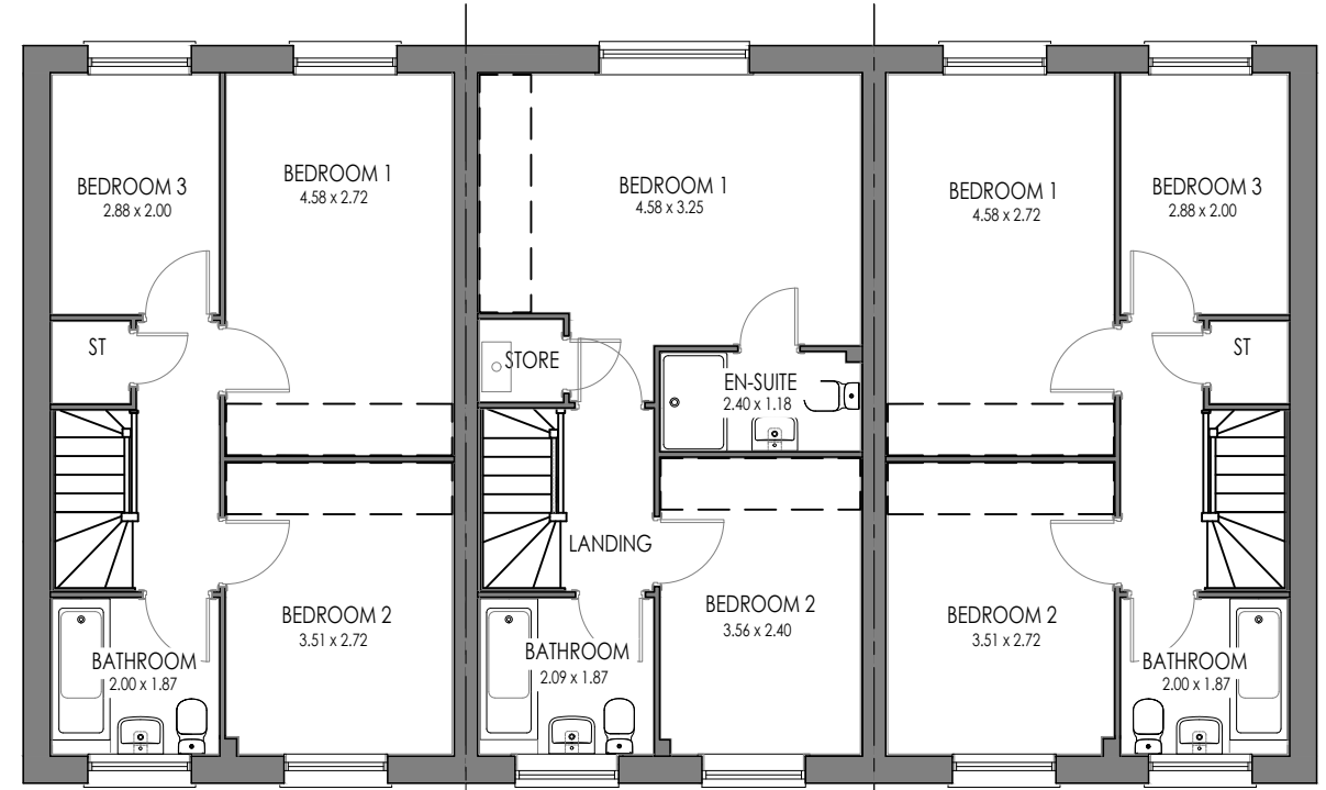
WARWICK (AS) FIRST FLOOR
