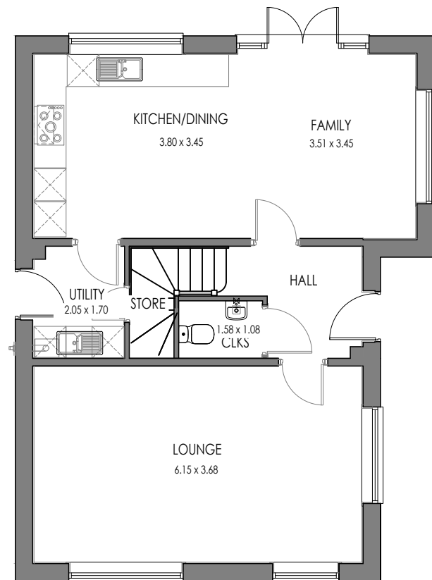
HEATHERINGTON (AS) GROUND FLOOR
