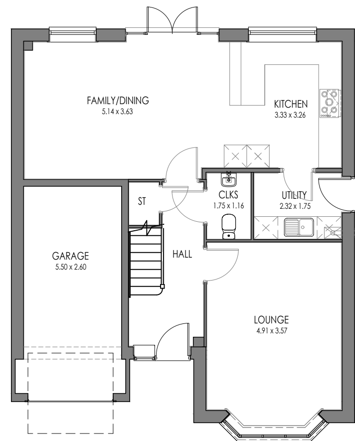
ALDERTON (AS) GROUND FLOOR
