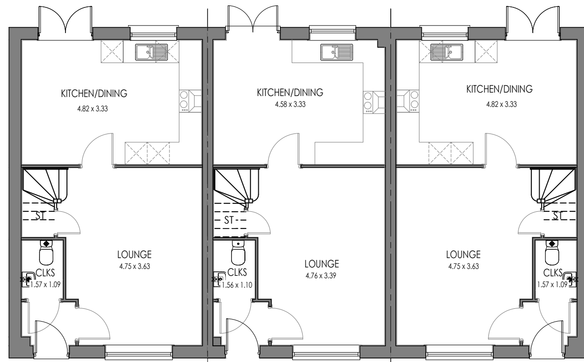
WARWICK (AS) GROUND FLOOR
