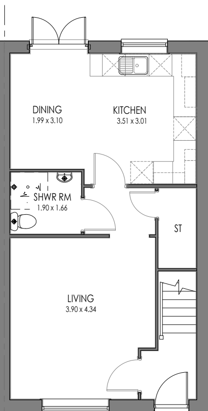
5P3B END (OPP) GROUND FLOOR
