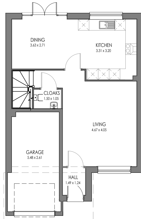
EVESHAM (AS) GROUND FLOOR
