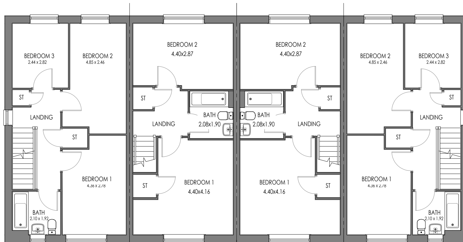
FIRST FLOOR 5P3B END (AS)
