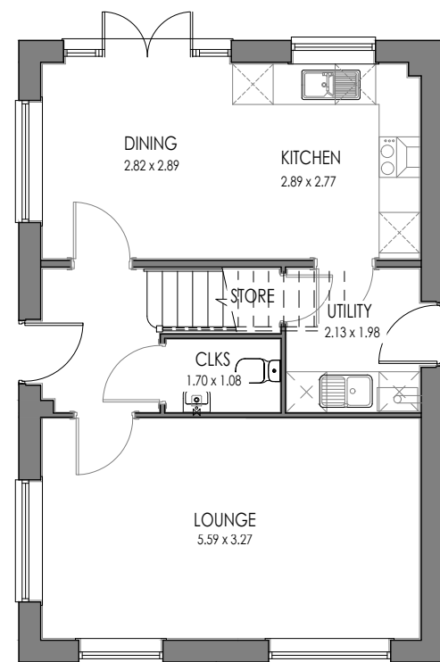
GROUND FLOOR HENLEY (AS)
