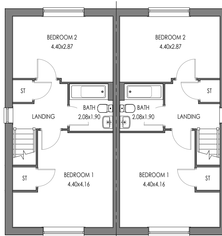
FIRST FLOOR 4P2B END (AS)
