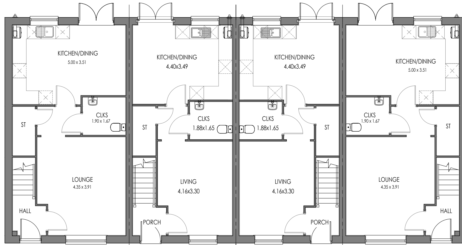
GROUND FLOOR 5P3B END (AS)
