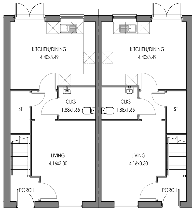
GROUND FLOOR 4P2B END (AS)
