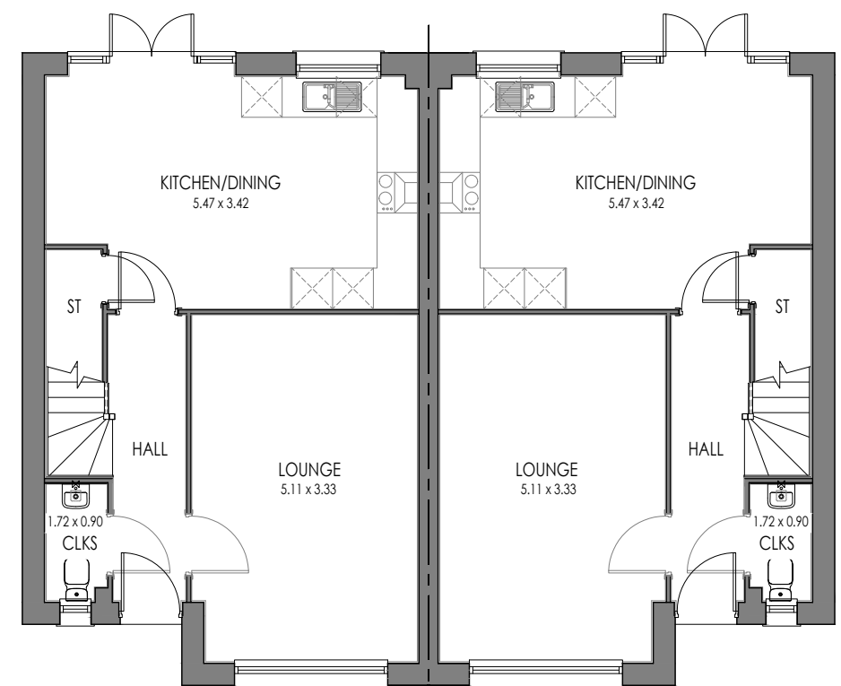
GROUND FLOOR MARLOW SEMI (AS)
