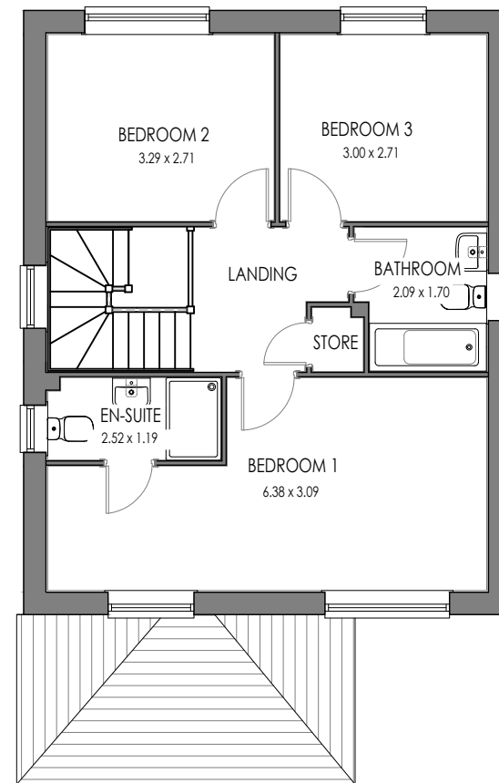
FIRST FLOOR PLAN STRATFORD (AS)
