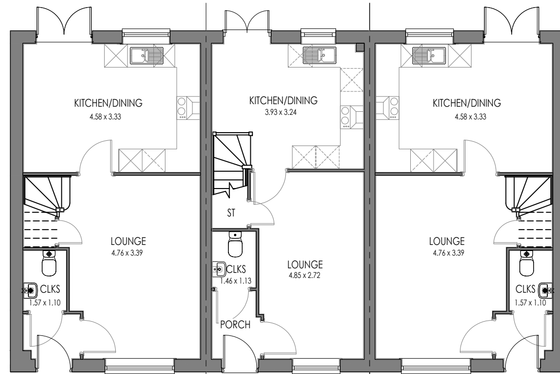
GROUND FLOOR HIGHFIELD (AS)
