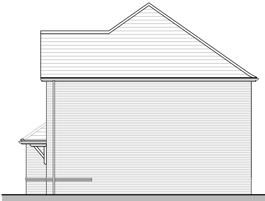
SIDE ELEVATION CHELTENHAM (AS)
