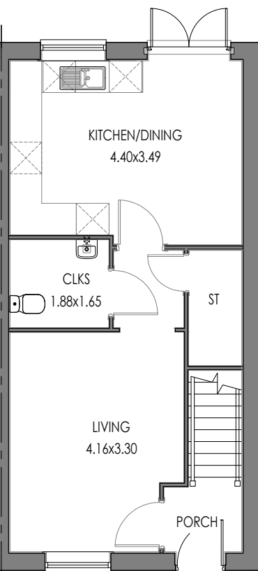
GROUND FLOOR 4P2B END (OPP)
