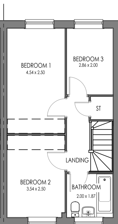
FIRST FLOOR HIGHFIELD (OPP)
