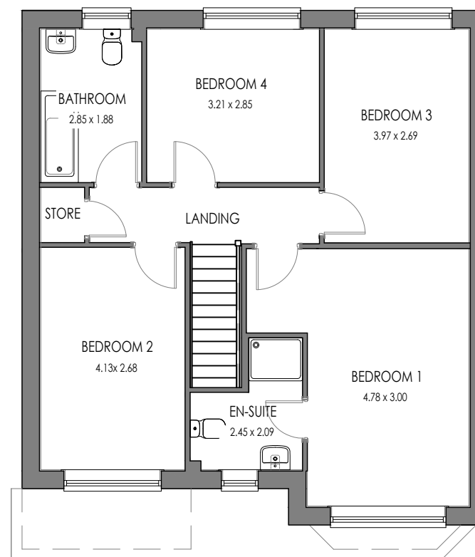
FIRST FLOOR WENTWORTH (AS)
