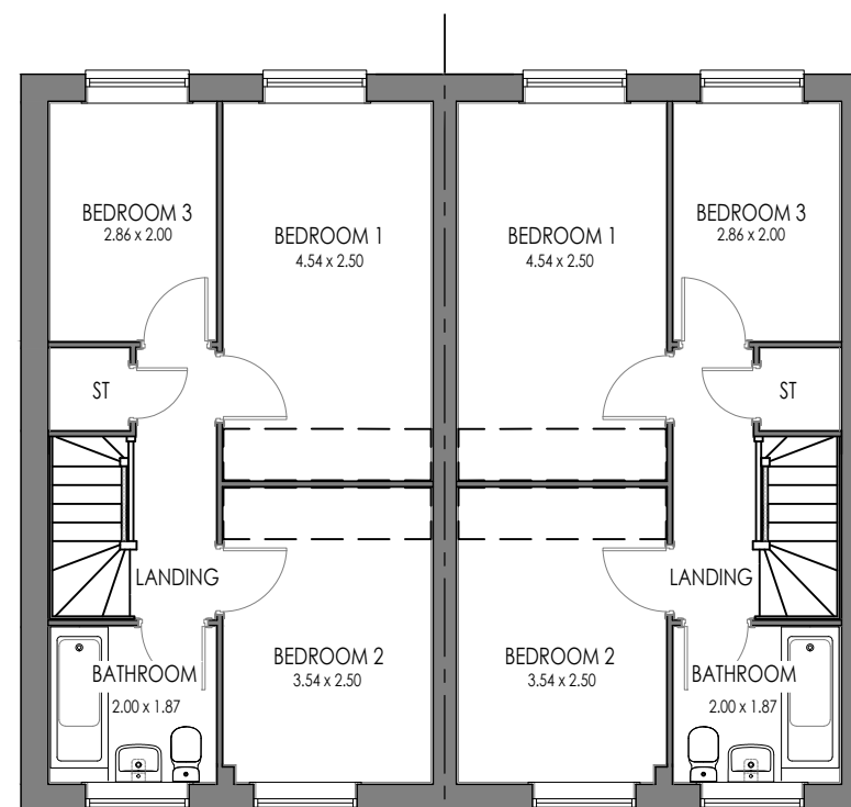
FIRST FLOOR HIGHFIELD (AS)
