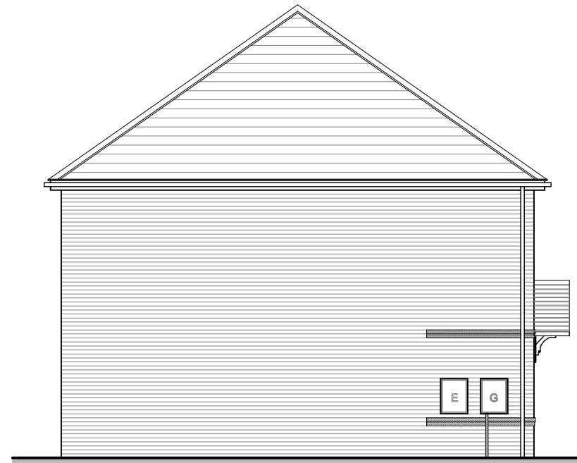
SIDE ELEVATION HIGHFIELD (AS)
