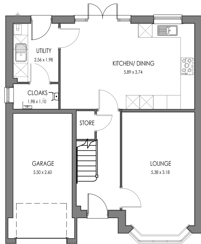
GROUND FLOOR WENTWORTH (AS)
