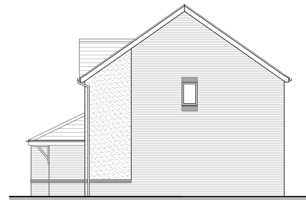
SIDE ELEVATION STRATFORD (AS)
