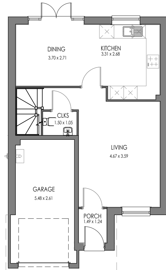
GROUND FLOOR PLAN STRATFORD (AS)
