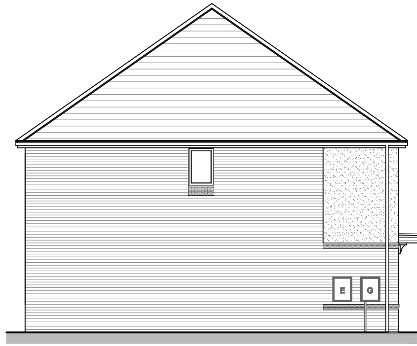
SIDE ELEVATION 4P2B END (AS)
