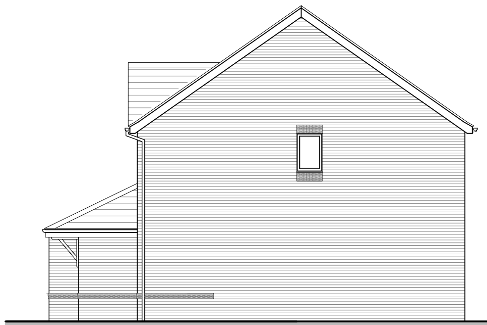
SIDE ELEVATION STRATFORD (AS)
