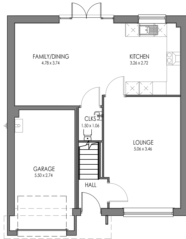
GROUND FLOOR CHELTENHAM (AS)
