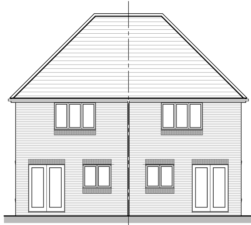
REAR ELEVATION 4P2B END (OPP)
