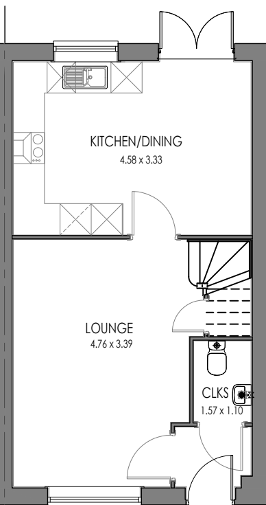
GROUND FLOOR HIGHFIELD (OPP)
