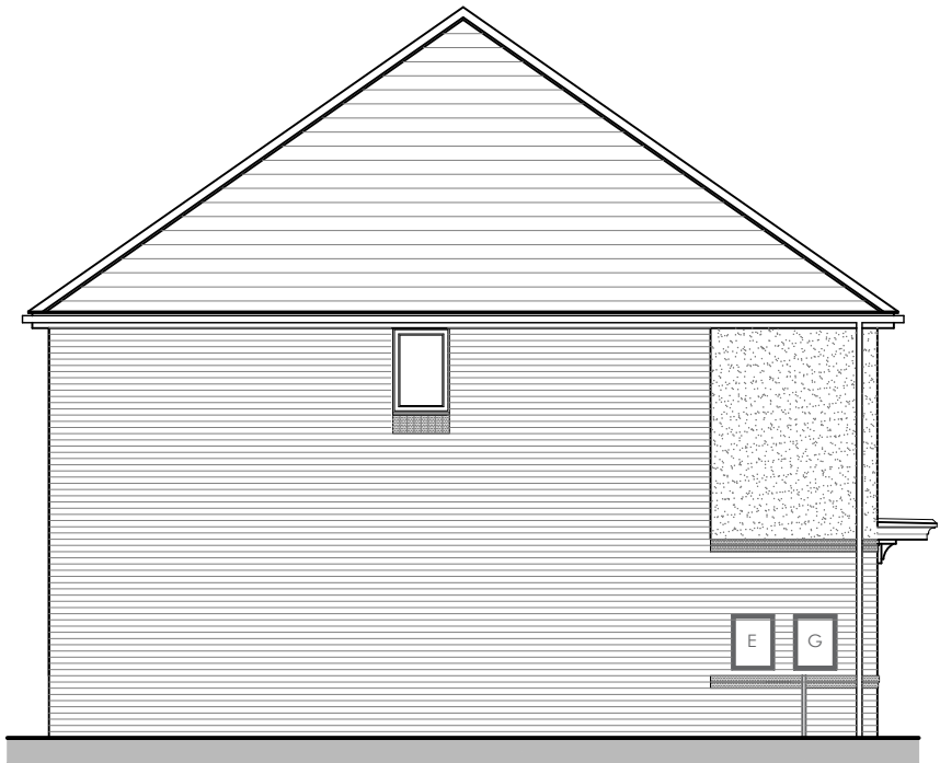
SIDE ELEVATION 5P3B END (AS)
