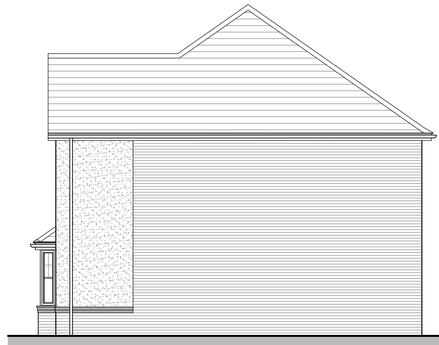
SIDE ELEVATION WENTWORTH (AS)
