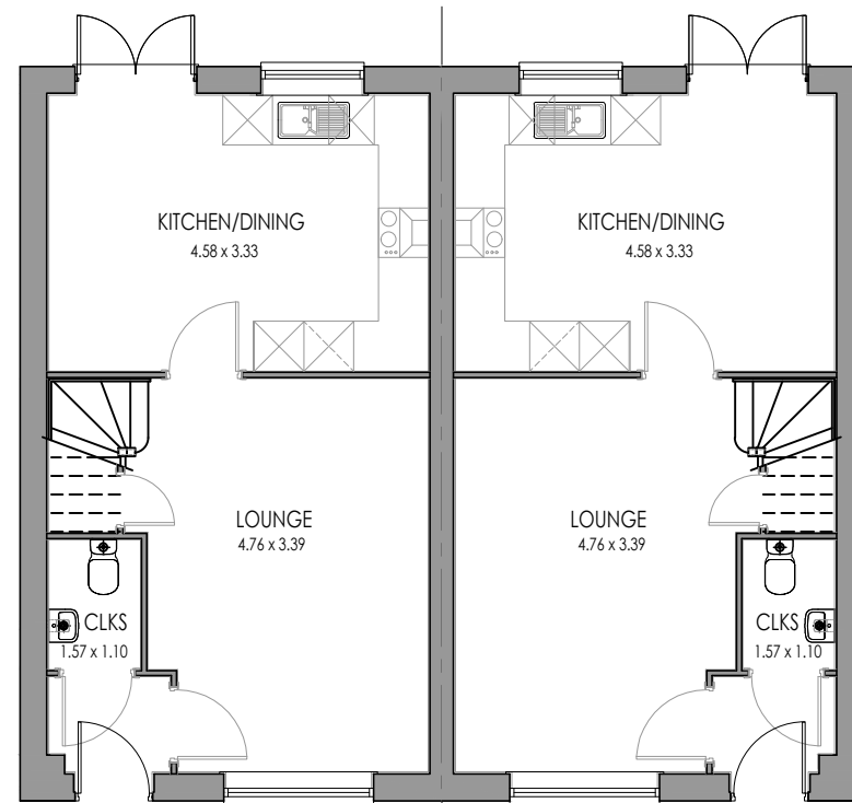
HIGHFIELD AS GROUND FLOOR
