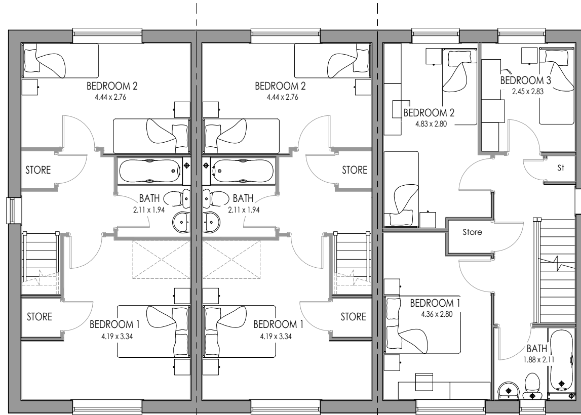
4P2B END AS FIRST FLOOR
