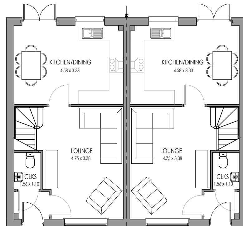
ASHTON AS GROUND FLOOR
