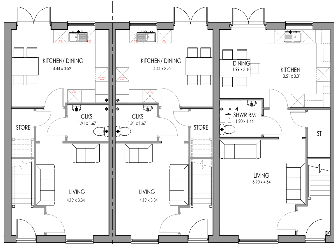
4P2B END AS GROUND FLOOR
