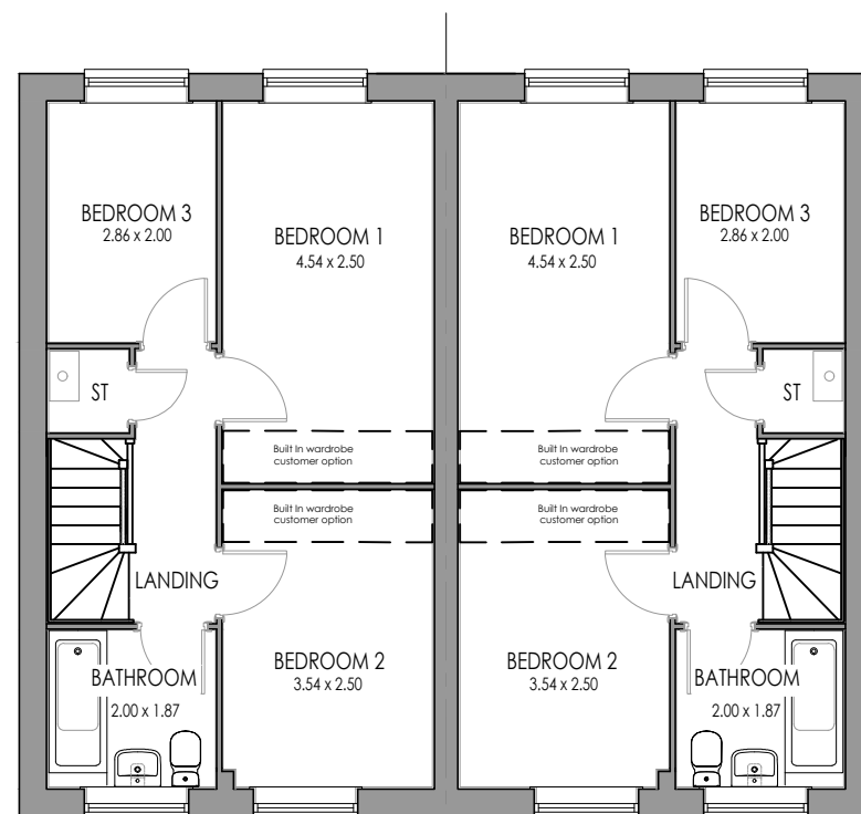
HIGHFIELD AS FIRST FLOOR
