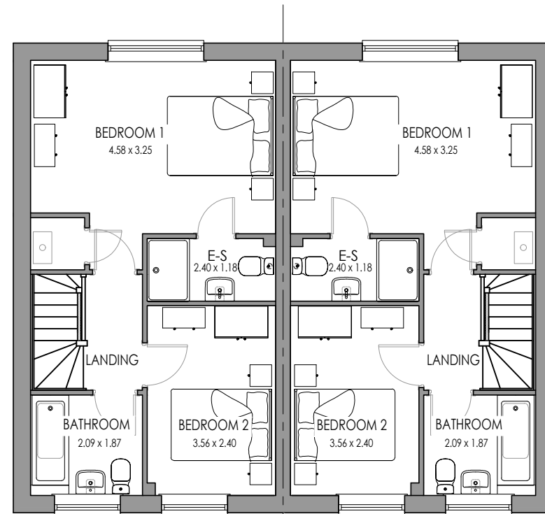
ASHTON AS FIRST FLOOR
