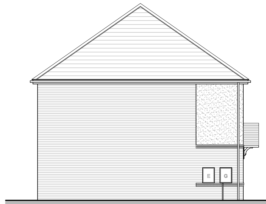
SIDE ELEVATION HR1 ASHTON AS
