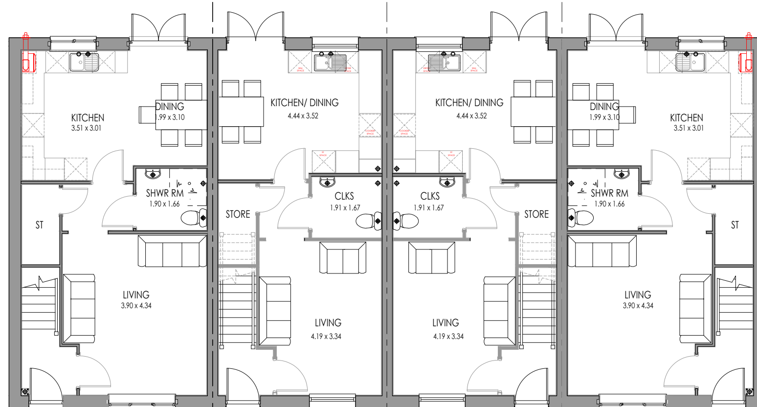
5P3B END AS GROUND FLOOR
