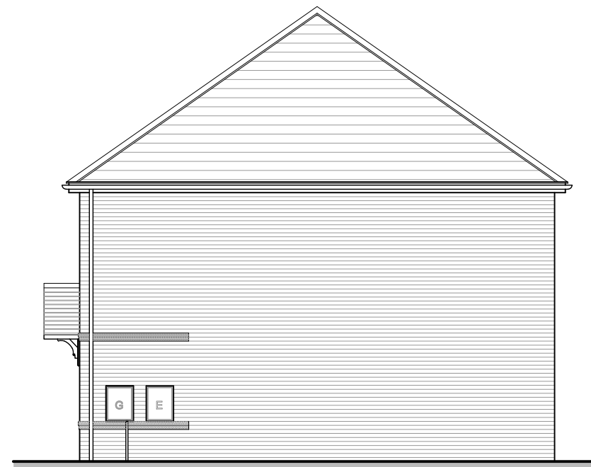
ELWY OPP SIDE ELEVATION
