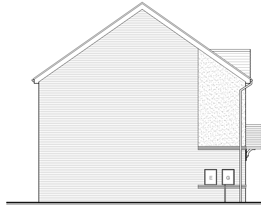
ELWY GR1 AS SIDE ELEVATION
