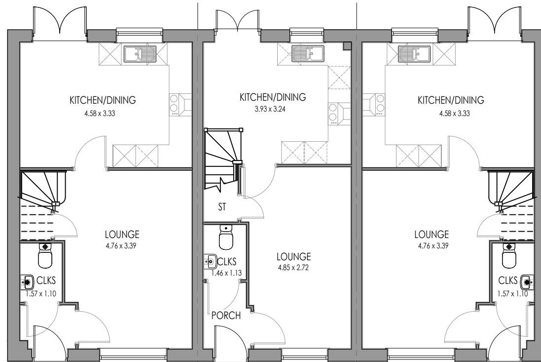
GROUND FLOOR
