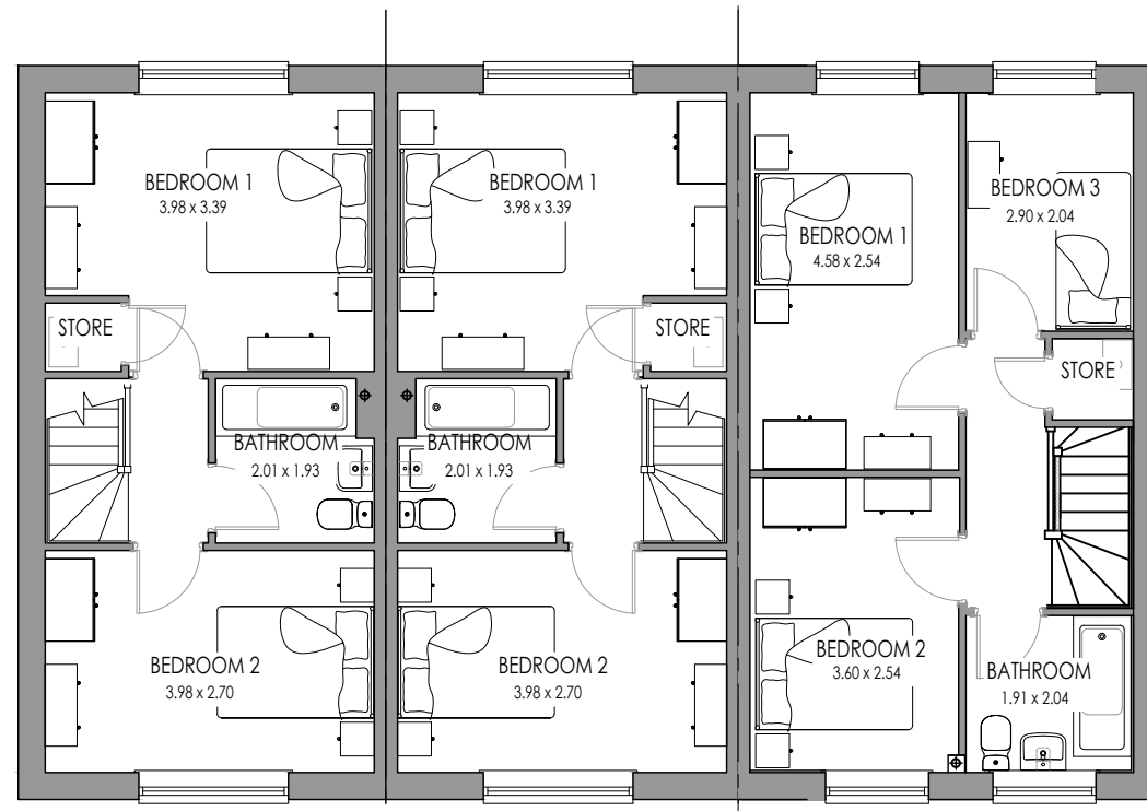
CLWYD AS FIRST FLOOR
