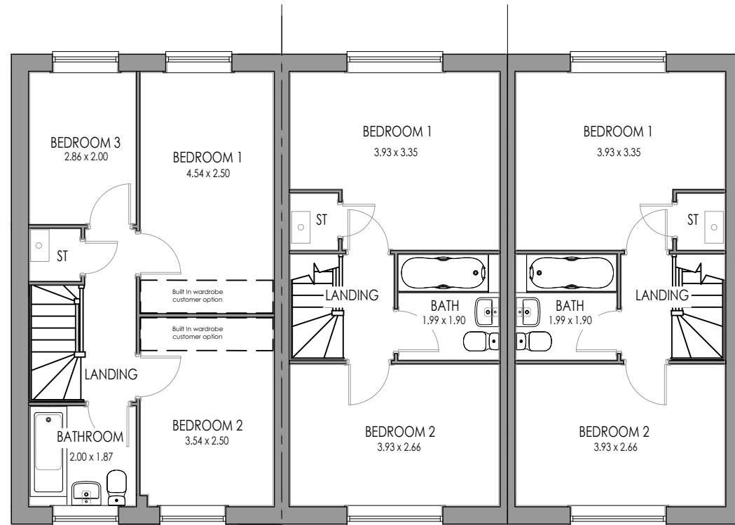
FIRST FLOOR
