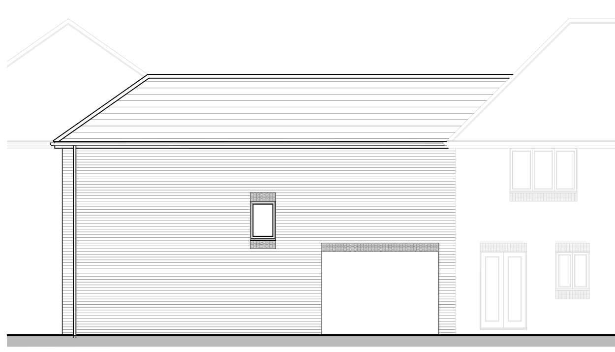
REAR ELEVATION
