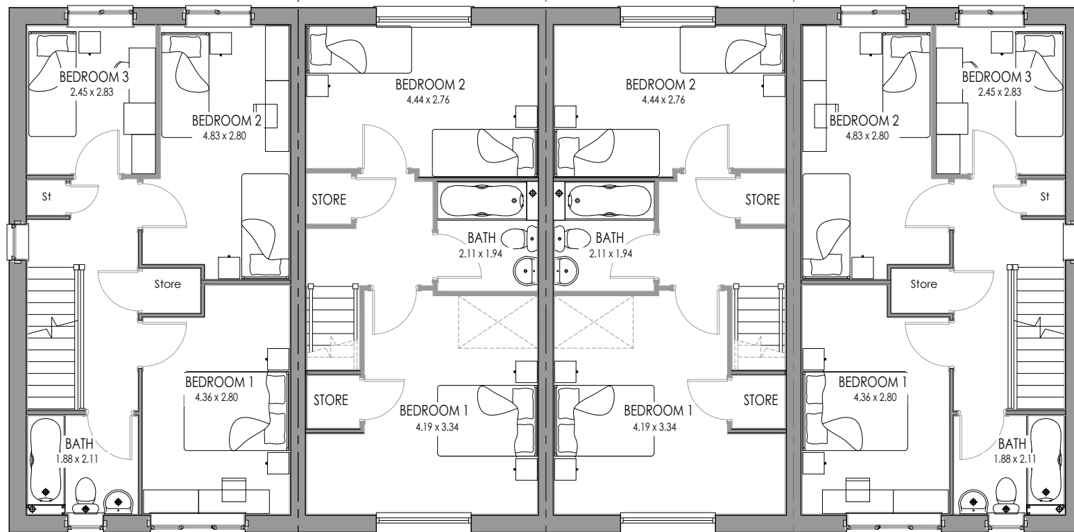
5P3B END AS FIRST FLOOR
