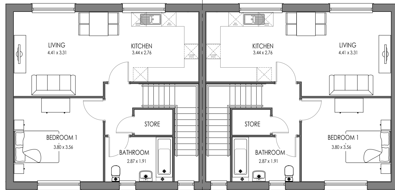
2B1P AS FIRST FLOOR
