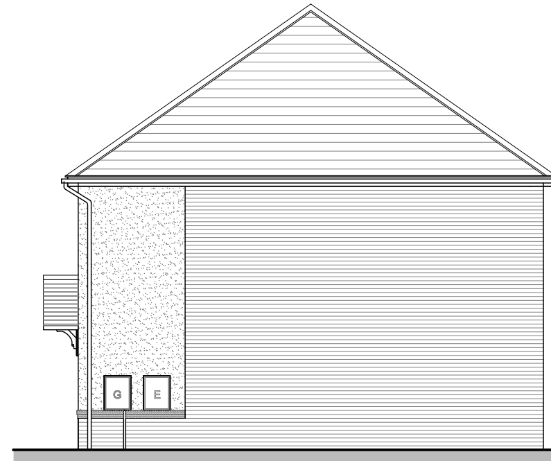
SIDE ELEVATION HR2 HIGHFIELD OPP
