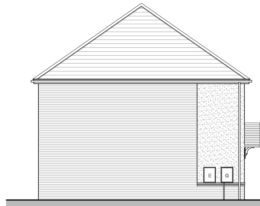
SIDE ELEVATION HR2 ASHTON OPP
