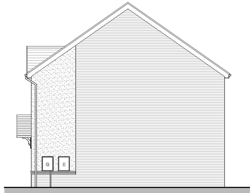
SIDE ELEVATION GR2 HIGHFIELD OPP
