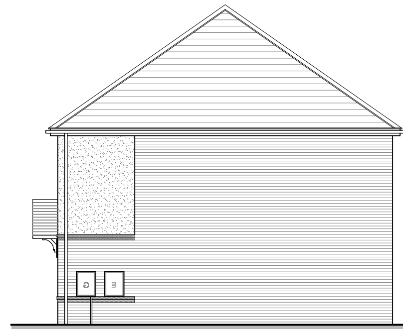
SIDE ELEVATION HR1 ASHTON OPP
