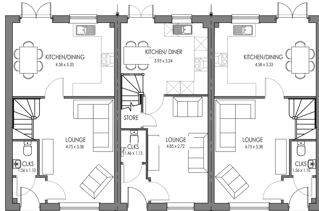
ASHTON AS GROUND FLOOR
