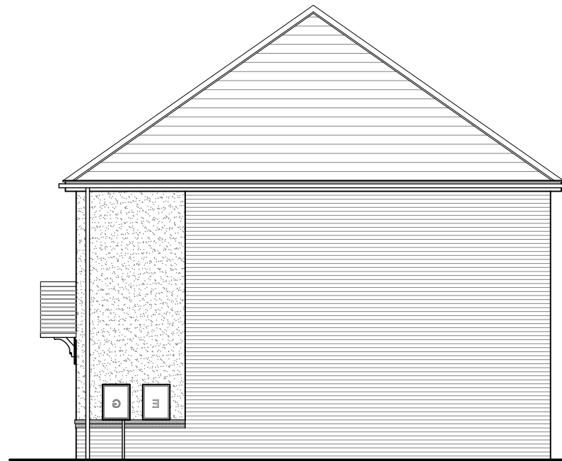
SIDE ELEVATION HR2 ASHTON OPP
