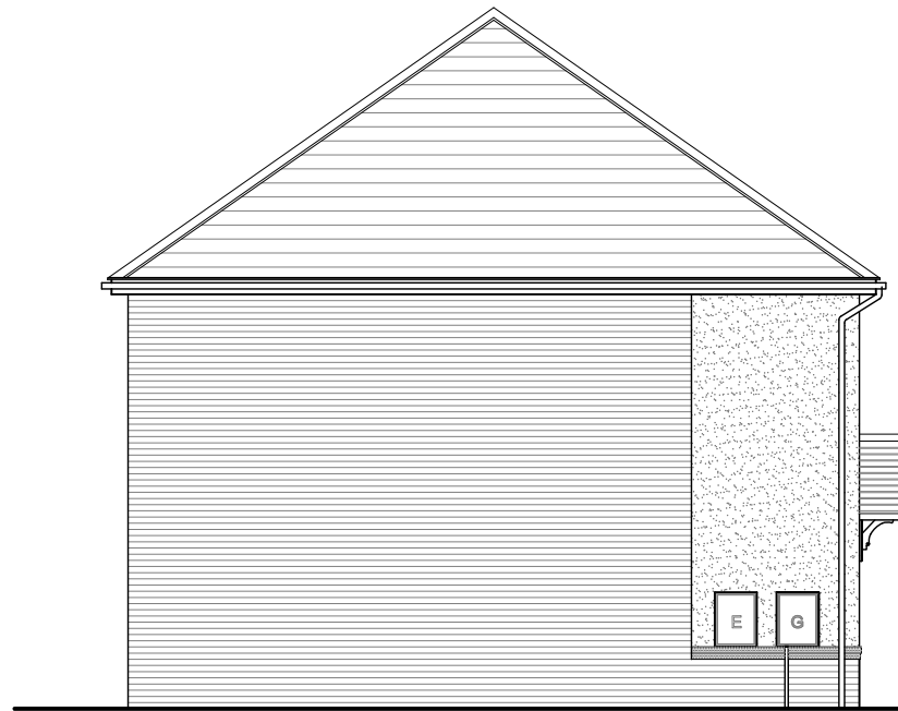
SIDE ELEVATION HR2 HIGHFIELD AS
