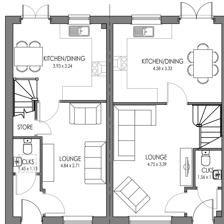
OAKLEY AS GROUND FLOOR
