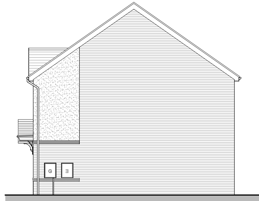
SIDE ELEVATION GR1
