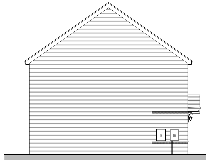
OAKLEY SIDE ELEVATION GB1
