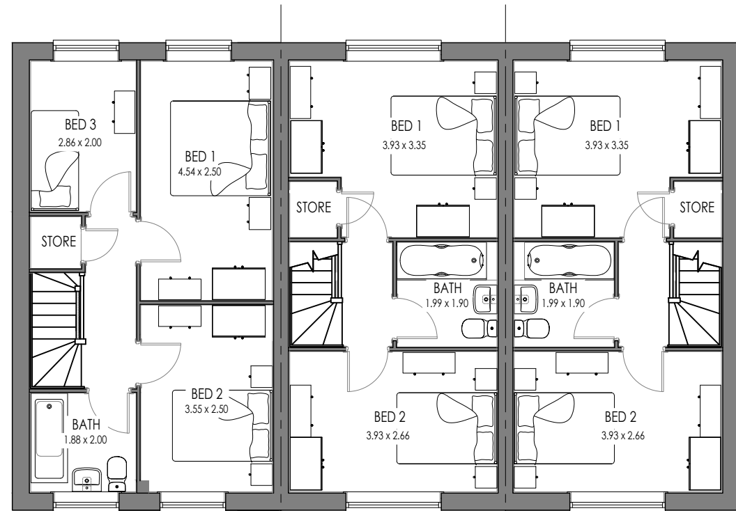
HIGHFIELD AS FIRST FLOOR
