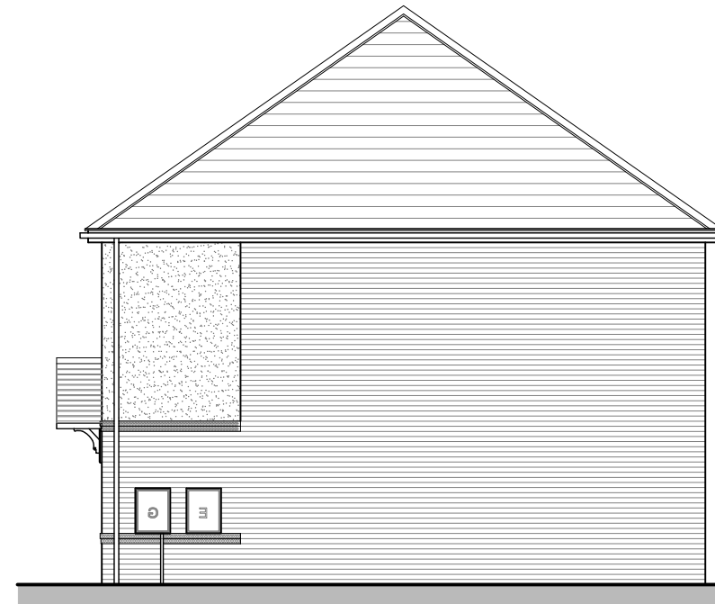
SIDE ELEVATION HR1 ASHTON OPP
