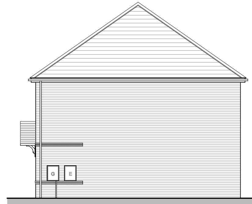
SIDE ELEVATION HB1 ASHTON OPP
