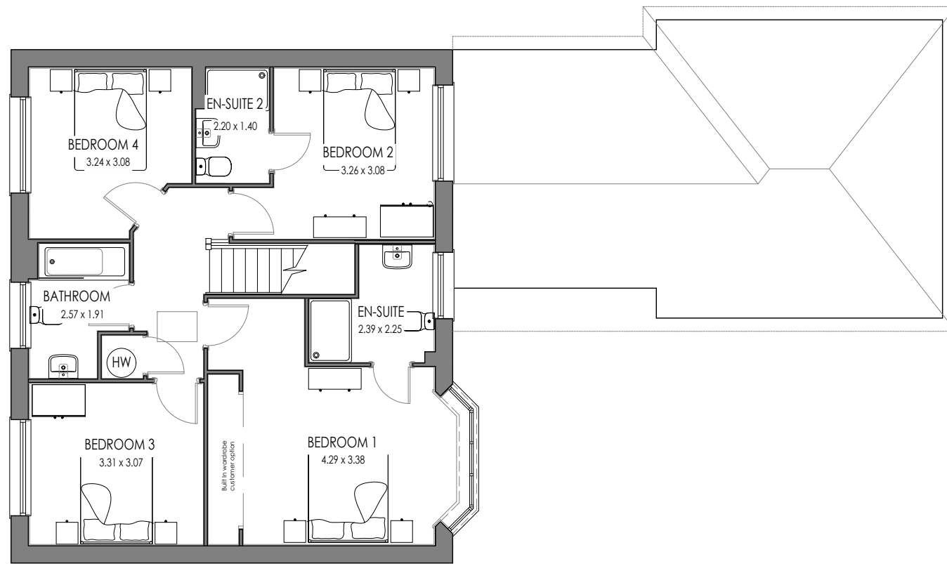
FIRST FLOOR
