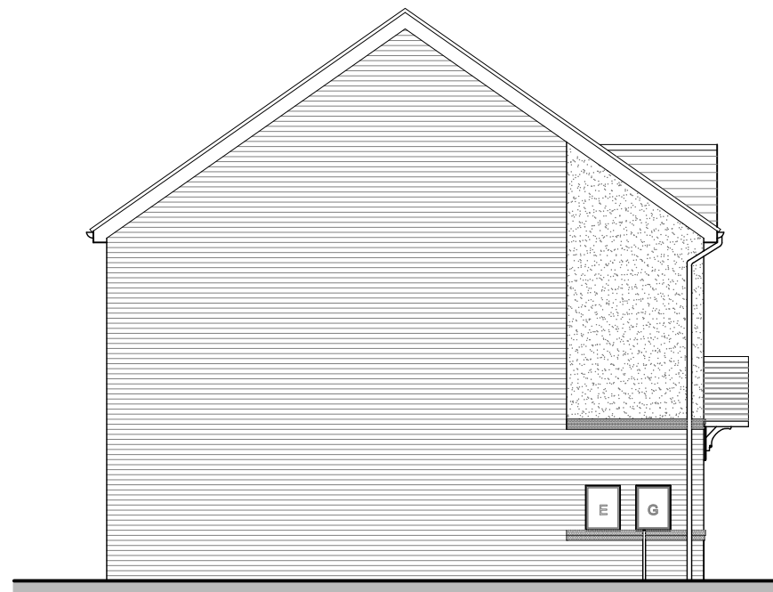
SIDE ELEVATION GR1 HIGHFIELD AS
