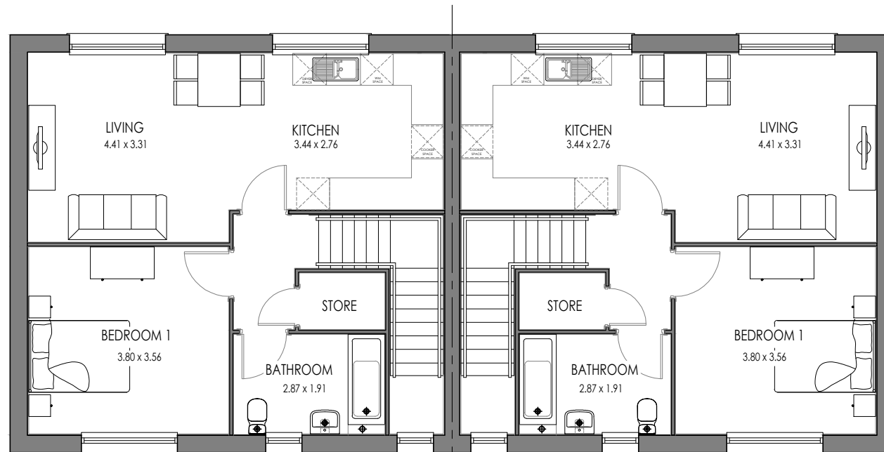
2B1P AS FIRST FLOOR
