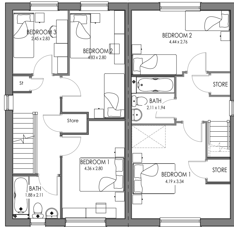
5P3B END AS FIRST FLOOR
