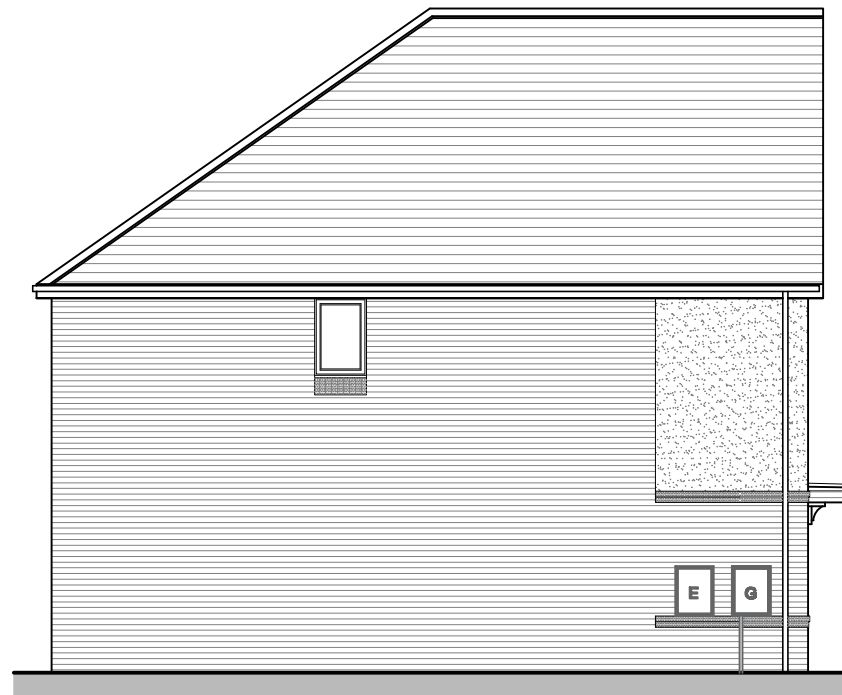
6P4B AS SIDE ELEVATION
