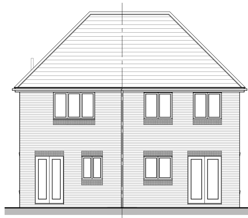
REAR ELEVATION OAKLEY OPP
