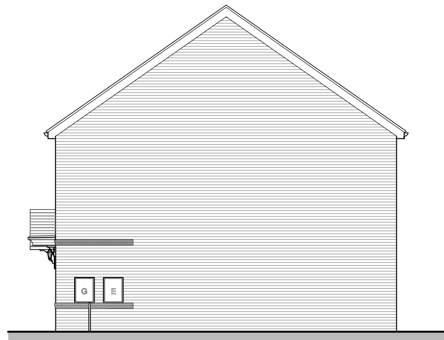
SIDE ELEVATION OAKLEY OPP
