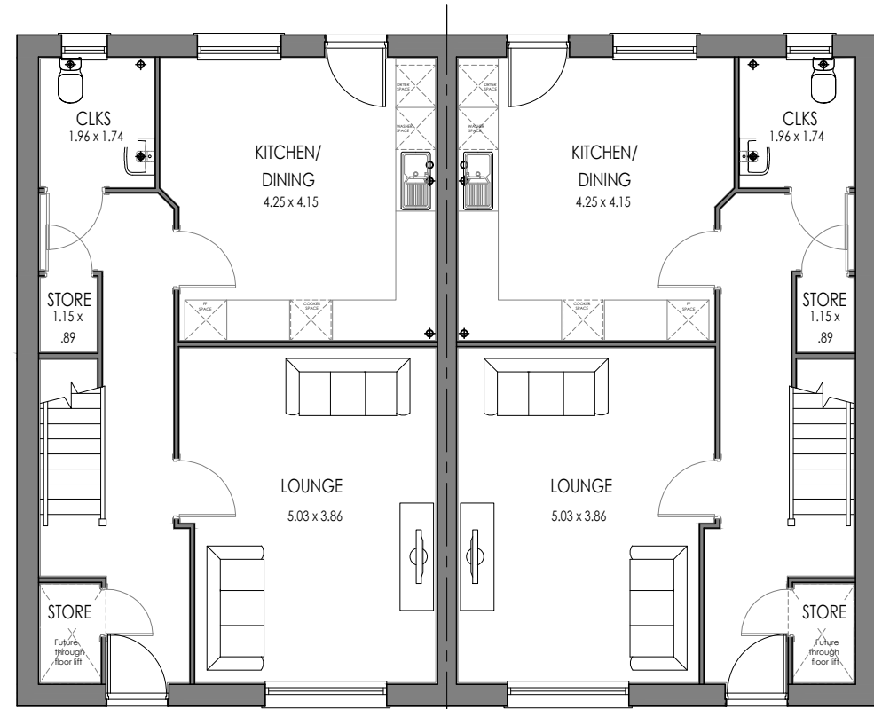
6P4B AS GROUND FLOOR
