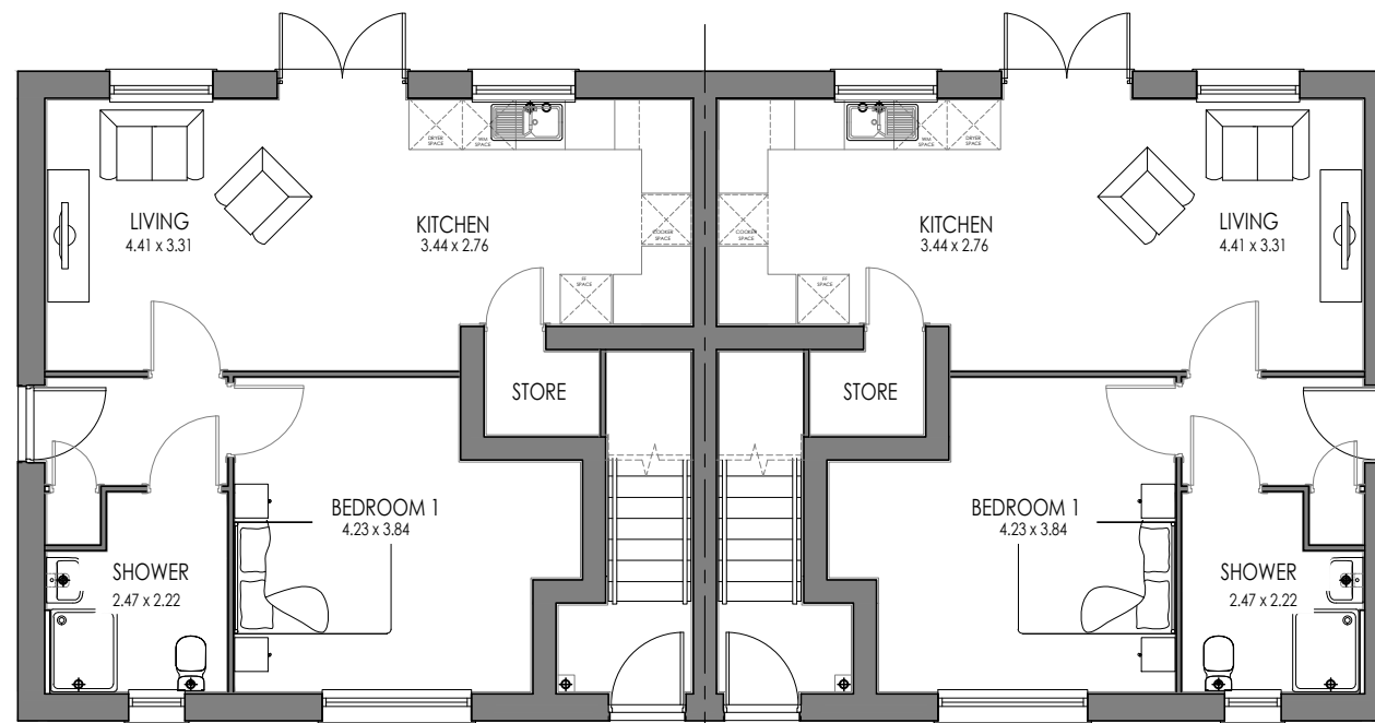
2P1B AS GROUND FLOOR
