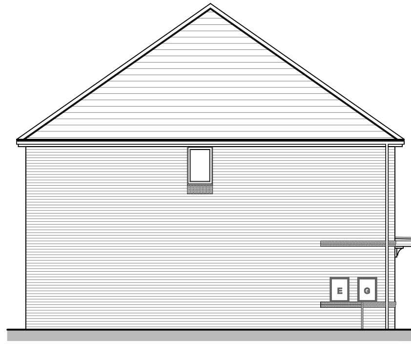
4P2B END AS SIDE ELEVATION
