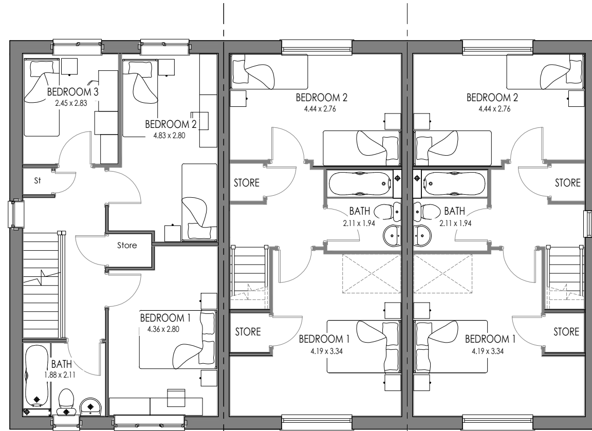
4P2B END OPP FIRST FLOOR
