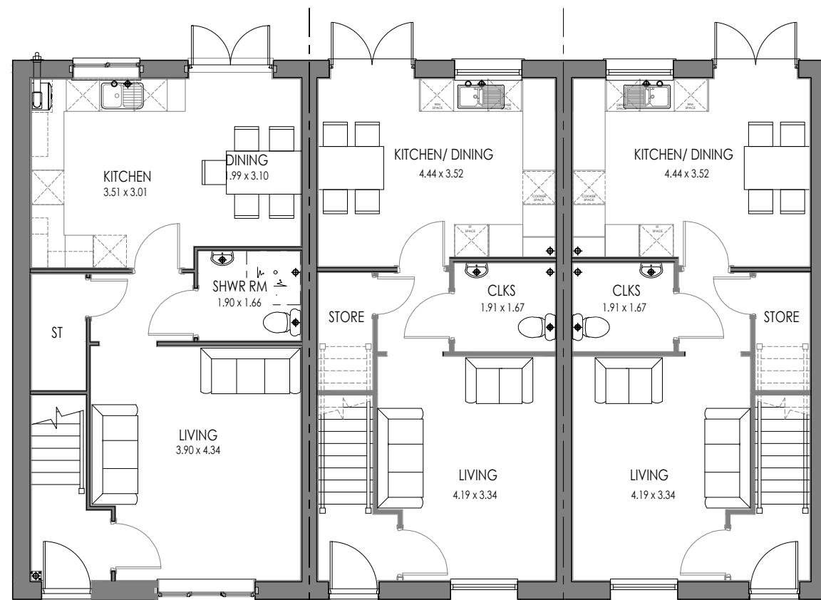
4P2B MID AS GROUND FLOOR
