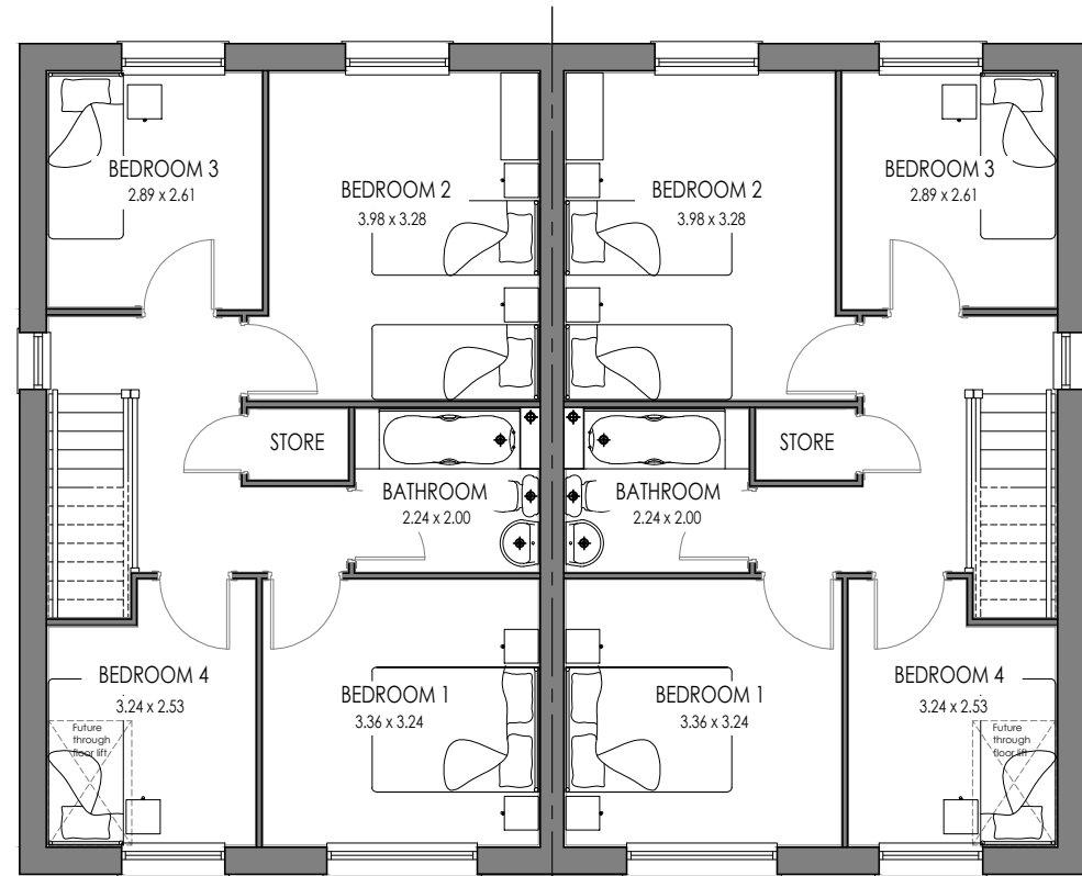
6P4B AS FIRST FLOOR
