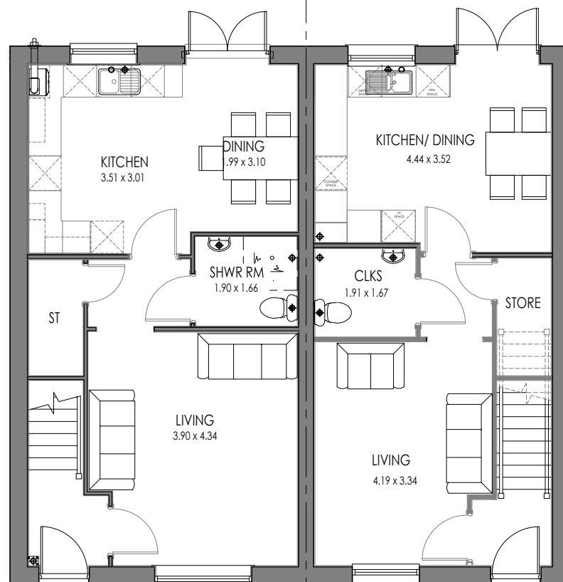
4P2B END OPP GROUND FLOOR
