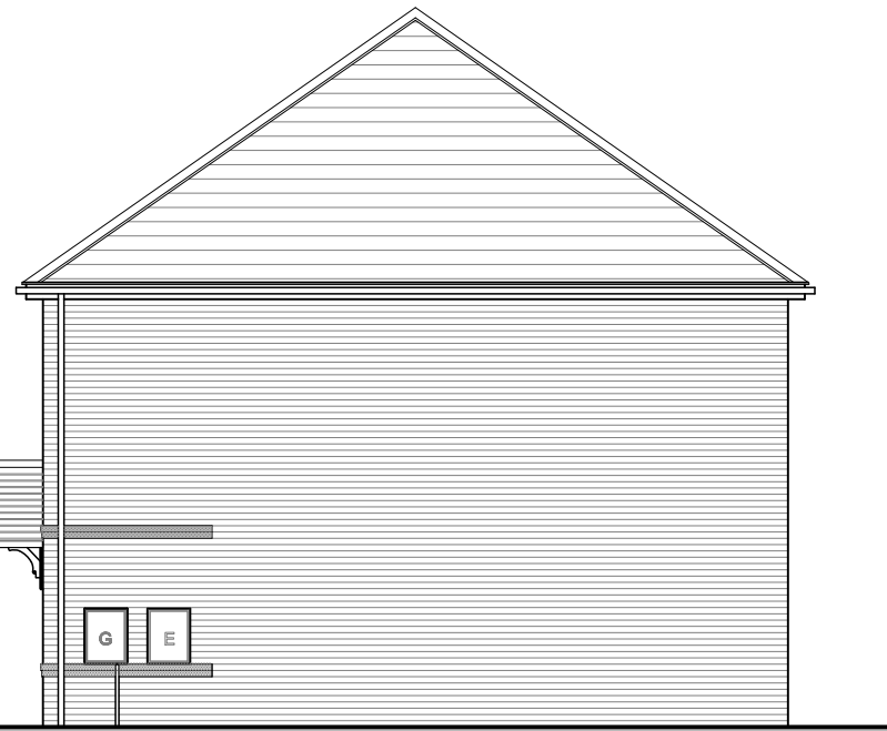
SIDE ELEVATION HIGHFIELD (HB1)
