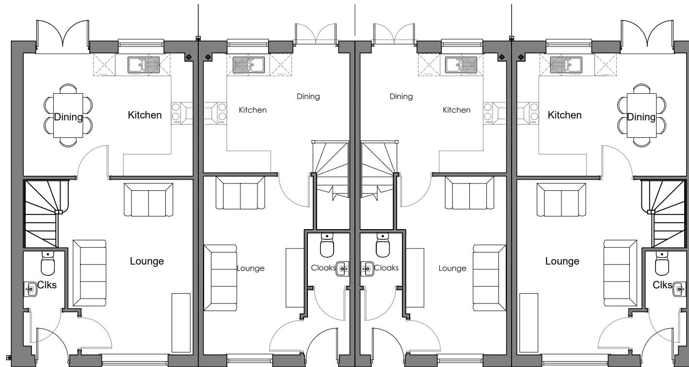
GROUND FLOOR HIGHFIELD
