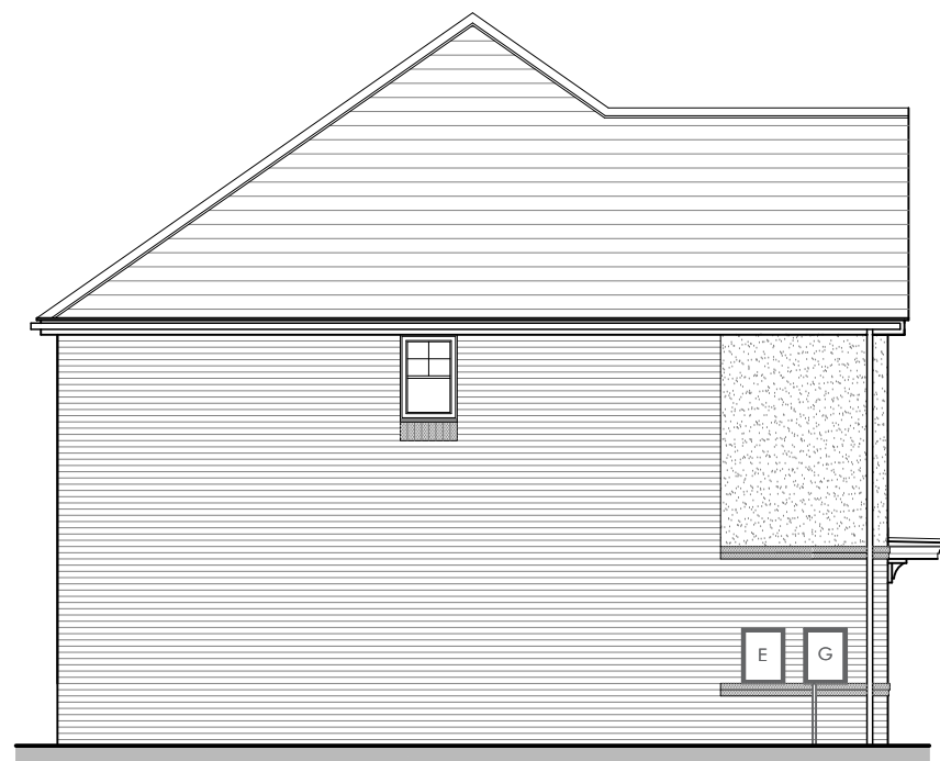
SIDE ELEVATION 5P3B (AS) PLOT 55
