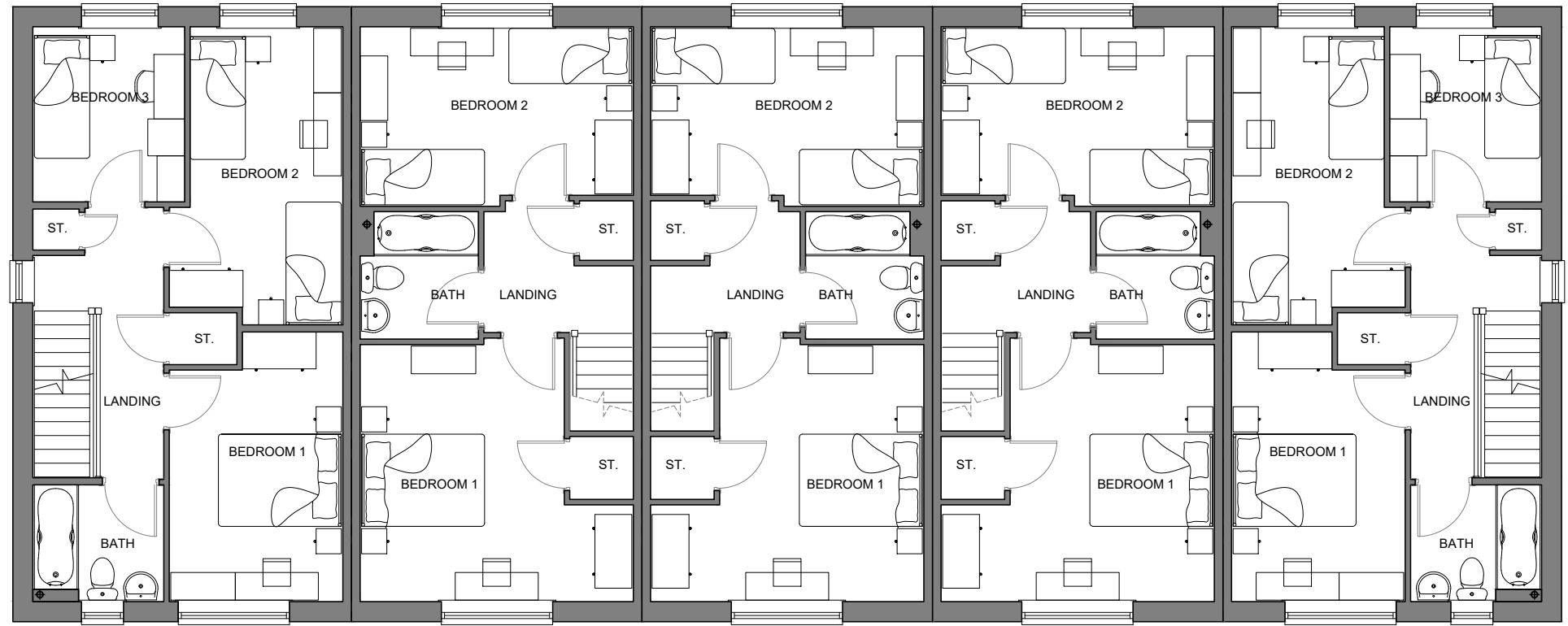
FIRST FLOOR 5P3B (AS) PLOT 20
