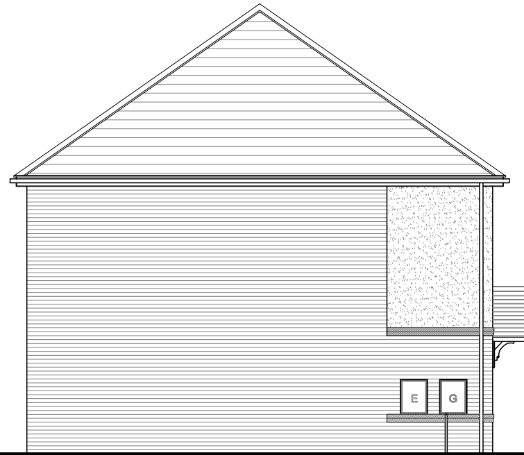
SIDE ELEVATION HIGHFIELD (HR1)
