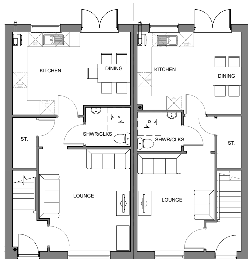
GROUND FLOOR 5P3B (AS) PLOT 20
