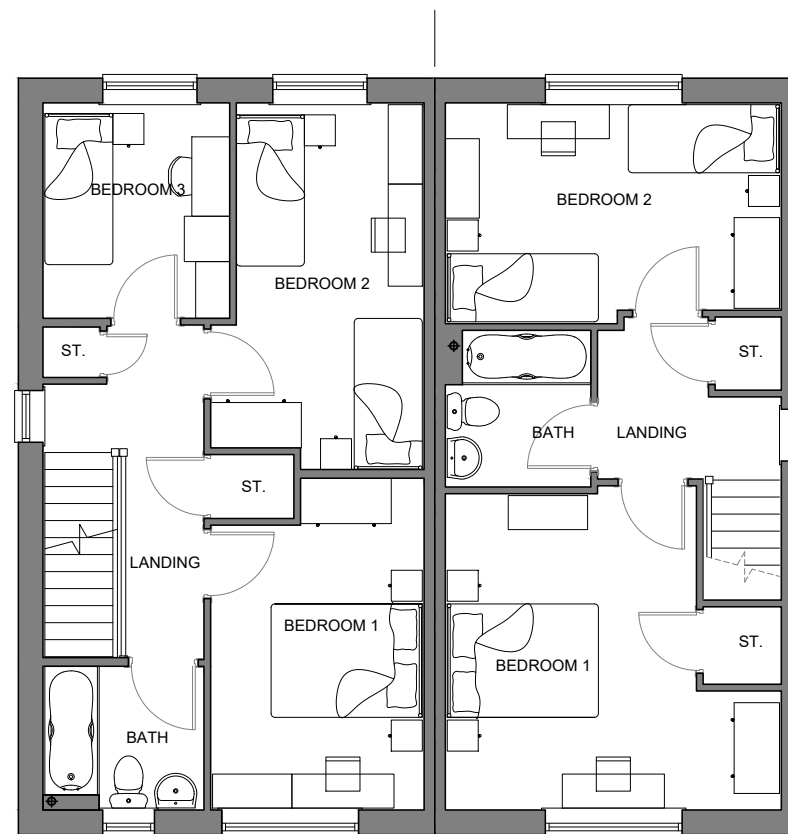
FIRST FLOOR 5P3B (AS) PLOT 20
