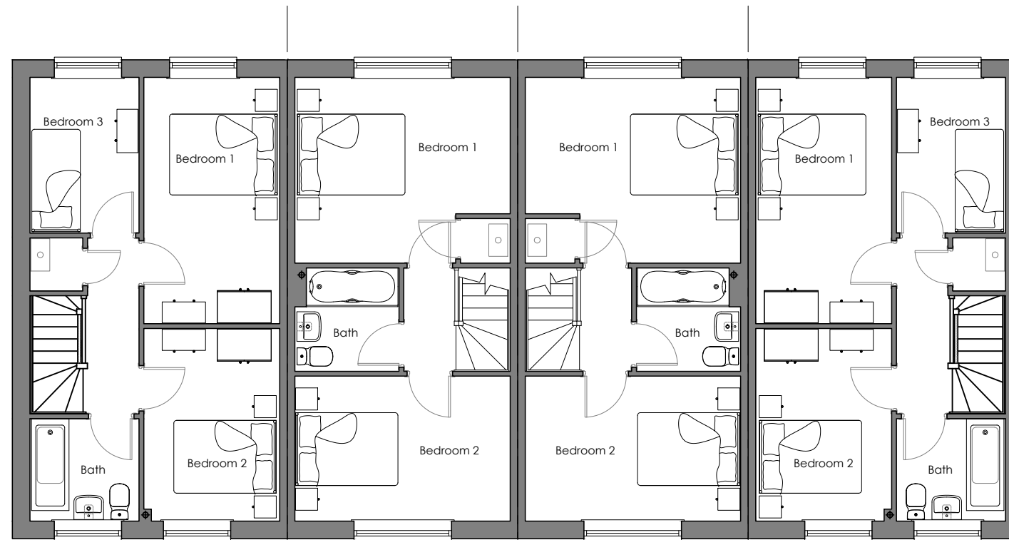
FIRST FLOOR HIGHFIELD
