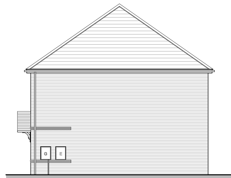
SIDE ELEVATION HIGHFIELD (HB1) PLOT 34
