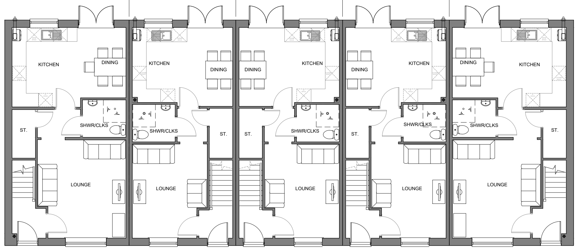
GROUND FLOOR 5P3B (AS) PLOT 20
