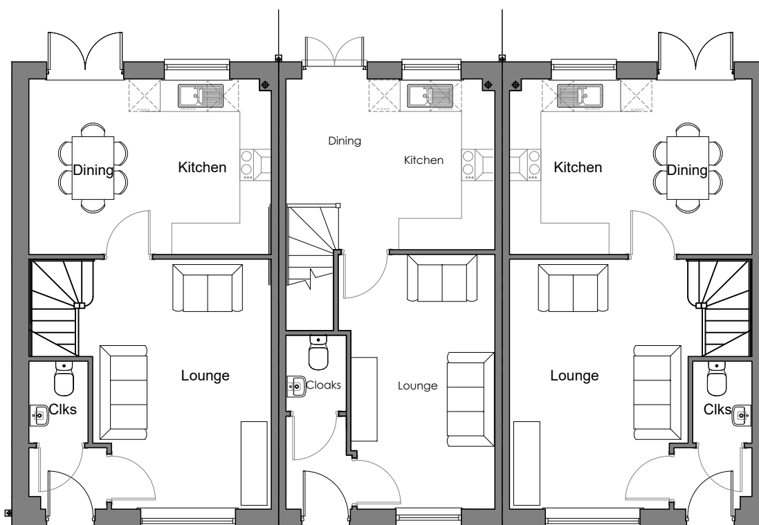
GROUND FLOOR HIGHFIELD
