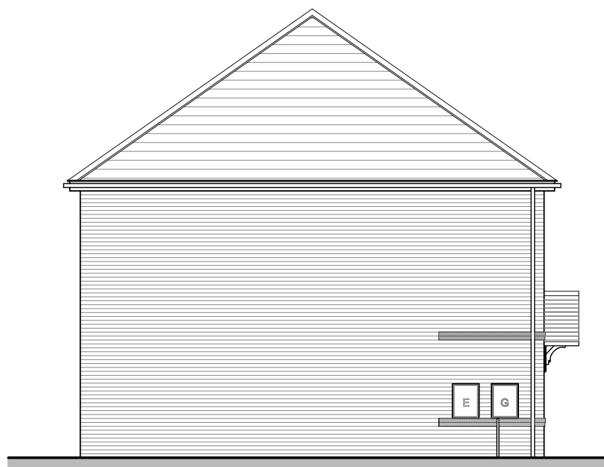
SIDE ELEVATION HIGHFIELD (HB1) PLOT 32
